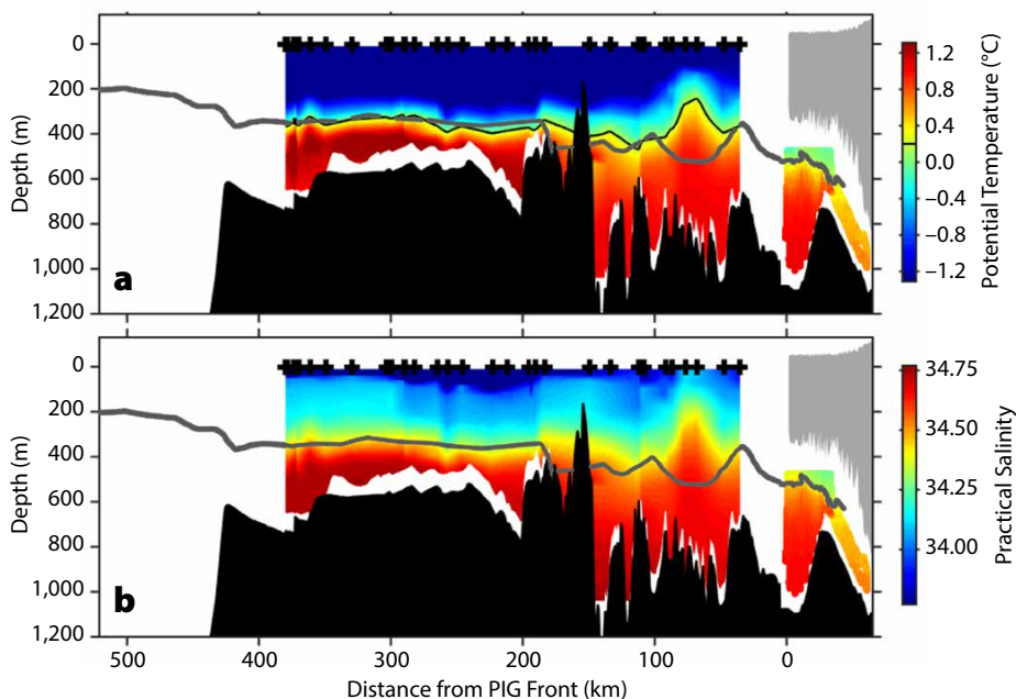
FIGURE 5. As Figure 4, but derived from seal-tag temperature and salinity profiles during February to April 2014. The data beneath Pine Island Glacier are the same as in Figure 4. The gray contour is the mid-thermocline isopycnal from the ship-based data as shown in Figure 4, to enable comparison.
