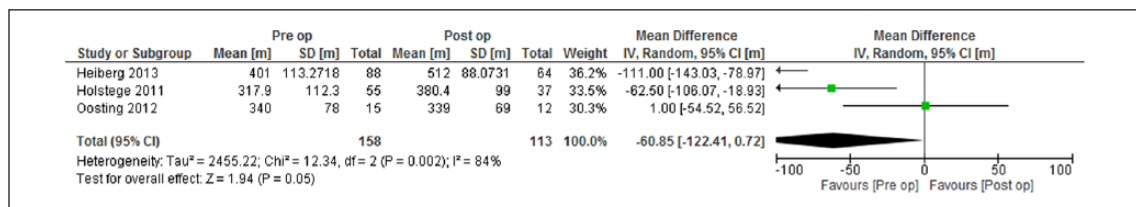
Figure 3. Random effects meta-analysis 6-minute walk test.
