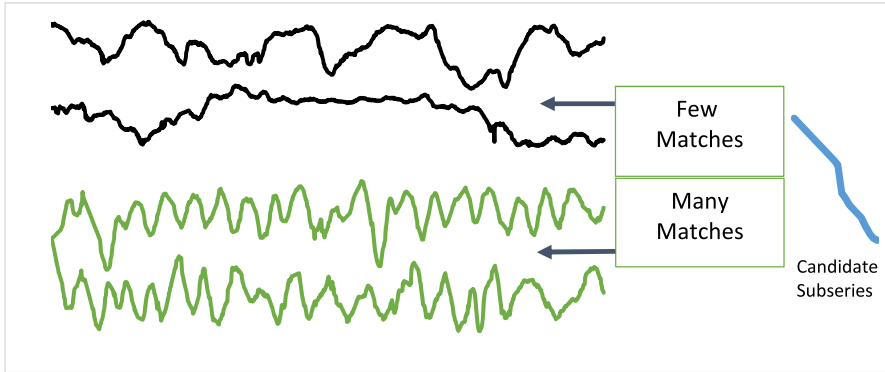
Fig. 6 An example of the need for detecting recurring patterns rather than unique patterns from WormsTwoClass. The top two series are the motion of normal worms, the bottom two mutant worms . The candidate subséries would not necessarily be a good shapelet, because there are close matches in both mutant and non mutant series
