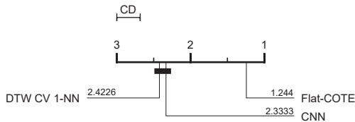
Fig. 2. Flat-COTE compared to DTW 1-NN and CNN.
