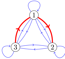
FIGURE 1. A graph showing that the condition that every vertex is the base of an RBR-circuit is not equivalent to saying that each vertex is contained in some RBR-alternating circuit. In all diagrams of graphs with red and blue edges, the red edges are drawn to be thicker than blue edges (for the convenience of readers with black and white copies of the article).
