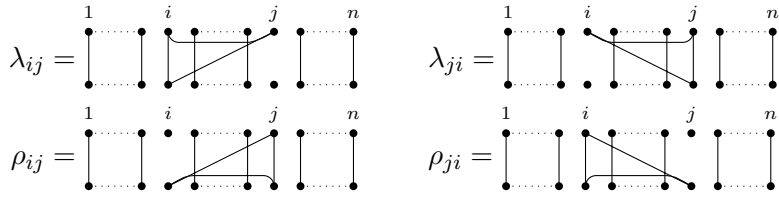
FIGURE 3. The non-projection idempotents of J_{n-1}(\mathcal{P}_n) ; see also Figure 2.
