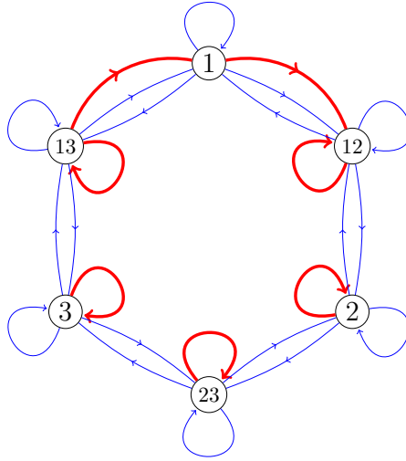
FIGURE 7. The digraph \Gamma_3(F) where F = \{\pi_2, \pi_3, \pi_{12}, \pi_{23}, \pi_{13}, \lambda_{31}, \rho_{12}\} in the partition monoid \mathcal{P}_3 .
