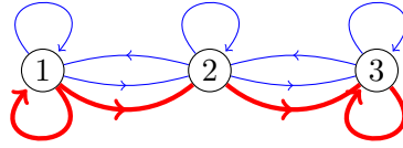
FIGURE 21. The digraph \Xi_4(F) , where F = \{\tau_1, \tau_3, \lambda_1, \lambda_2\} .
