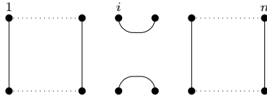
FIGURE 16. The projection \tau_i \in \mathcal{J}_n .
