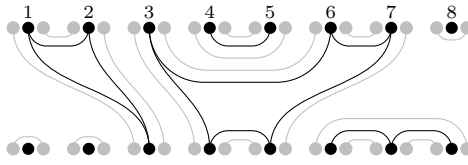
FIGURE 22. A planar partition from \mathcal{PP}_8 (black) and its image (gray) under the isomorphism \mathcal{PP}_8 \rightarrow \mathcal{J}_{16} .
