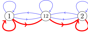
FIGURE 6. The digraph \Gamma_2(F) where F = \{\pi_1, \pi_2, \lambda_{12}, \rho_{12}\} in the partition monoid \mathcal{P}_2 .
