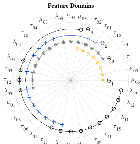
(c) Resulting feature domains.
