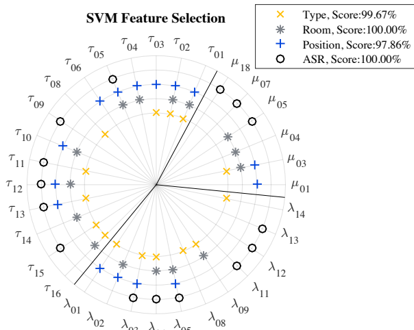
(b) Selected parameters for SVM using BSS.
