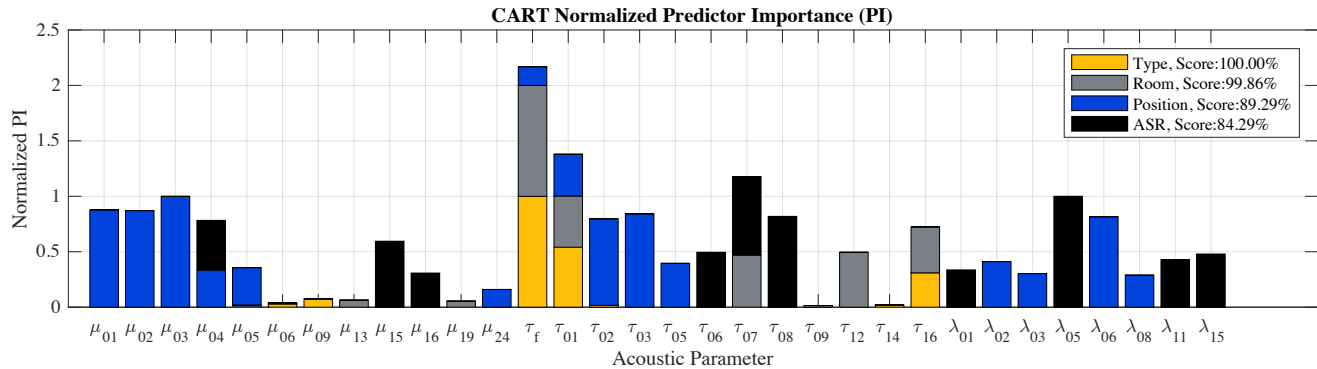
(a) Predictor Importance to CART growing.
