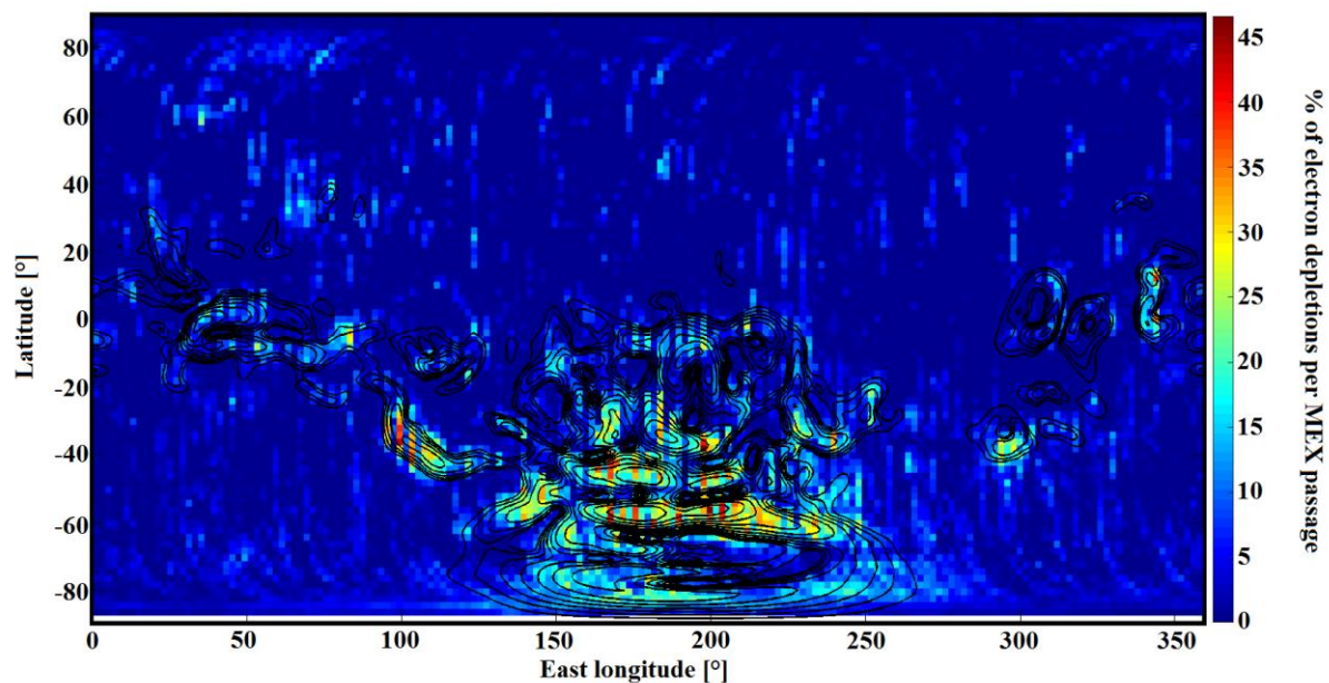
Figure 5: In color: Percentage of electron depletions detected with criterion (2) from MEX data per MEX passage on the nightside on a geographic map of the Martian surface with constant bin size of 2^\circ by 2^\circ . In black: horizontal magnetic field contour lines calculated from the model of Morschhauser at an altitude of 400 km. The contour lines have been plotted for horizontal crustal fields of: 10, 13, 16, 20, 25, 32, 40, 50, 63, 79 and 100 nT.
