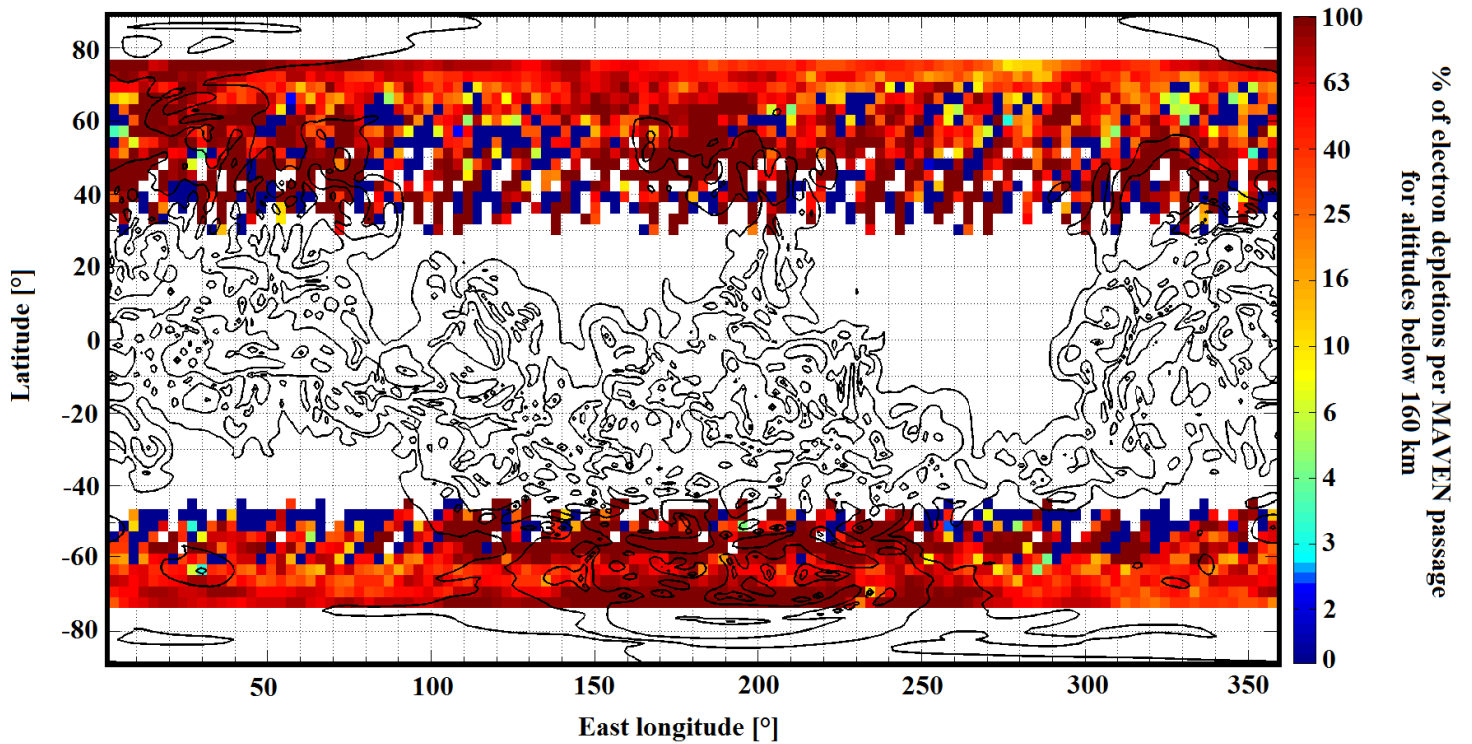
Figure 7: In color: Percentage of electron depletions detected below 160 km with criterion (1) from MAVEN data per MAVEN passage on the nightside on a geographic map of the Martian surface with constant bin size of 3^\circ by 3^\circ . In black: horizontal magnetic field contour lines calculated from the model of Morschhauser at an altitude of 170 km. The contour lines have been plotted for horizontal crustal fields of: 10, 32, 100, 316 and 1000 nT.
