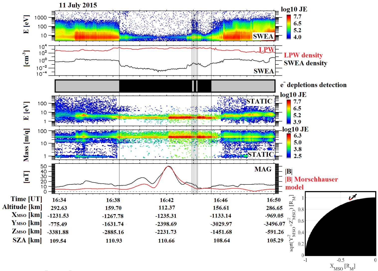
Figure 3. Example of electron depletion observed with MAVEN. First panel: SWEA energy-time spectrogram of omnidirectional electron energy flux (ENGY mode) corrected for the potential measured with LPW. Second panel: Electron density calculated with SWEA (black) superimposed with the density calculated with LPW (red). Third panel: Detection of electron depletions by criterion (1) (black boxes). See section 3 for more details. The shadow corresponds to the nightside. Fourth panel: STATIC energy-time spectrogram of omnidirectional ion energy flux (C0 mode). Fifth panel: STATIC mass-time spectrogram of omnidirectional ion energy flux (C6 mode). Sixth panel: Magnetic field intensity (measured by MAG in black and calculated from the model of Morschhauser in red). Seventh panel (bottom right): MAVEN orbital trajectory in a cylindrically symmetric MSO coordinates frame. The location of the electron depletions detected have been highlighted in red.
