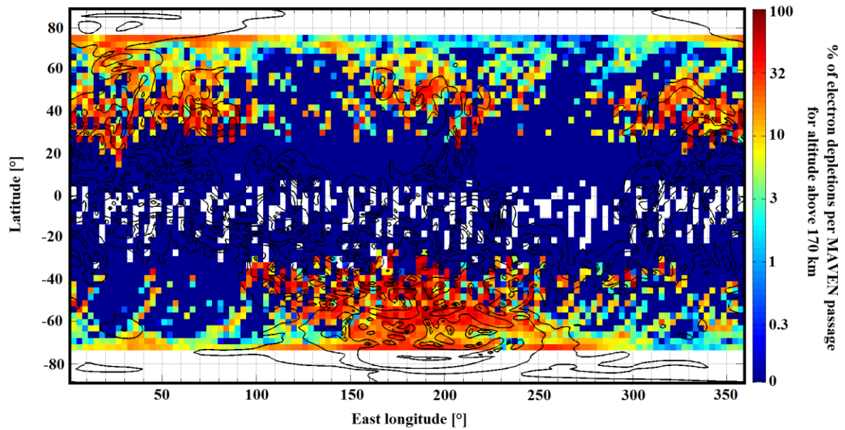
Figure 6: In color: Percentage of electron depletions detected above 170 km with criterion (1) from MAVEN data per MAVEN passage on the nightside on a geographic map of the Martian surface with constant bin size of 3^\circ by 3^\circ . In black: horizontal magnetic field contour lines calculated from the model of Morschhauser at an altitude of 170 km. The contour lines have been plotted for horizontal crustal fields of: 10, 32, 100, 316 and 1000 nT.
