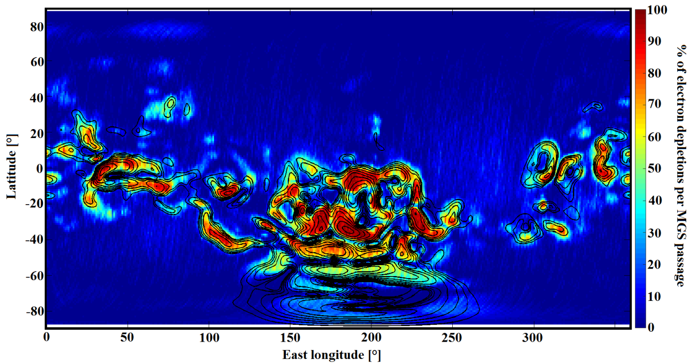
Figure 4. In color: Percentage of electron depletions detected with criterion (3) from MGS data per MGS passage on the nightside on a geographic map of the Martian surface with constant bin size of 1^\circ by 1^\circ . In black: horizontal magnetic field contour lines calculated from the model of Morschhauser at an altitude of 400 km. The contour lines have been plotted for horizontal crustal fields of: 10, 13, 16, 20, 25, 32, 40, 50, 63, 79 and 100 nT.
