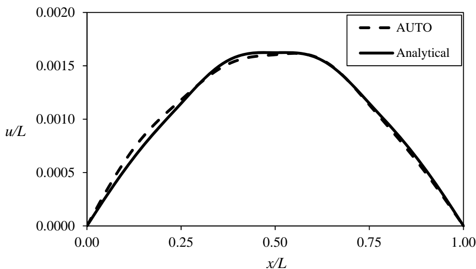
Figure 3: Typical comparison of analytical and numerical results for deflected shape for the linearly-elastic model
