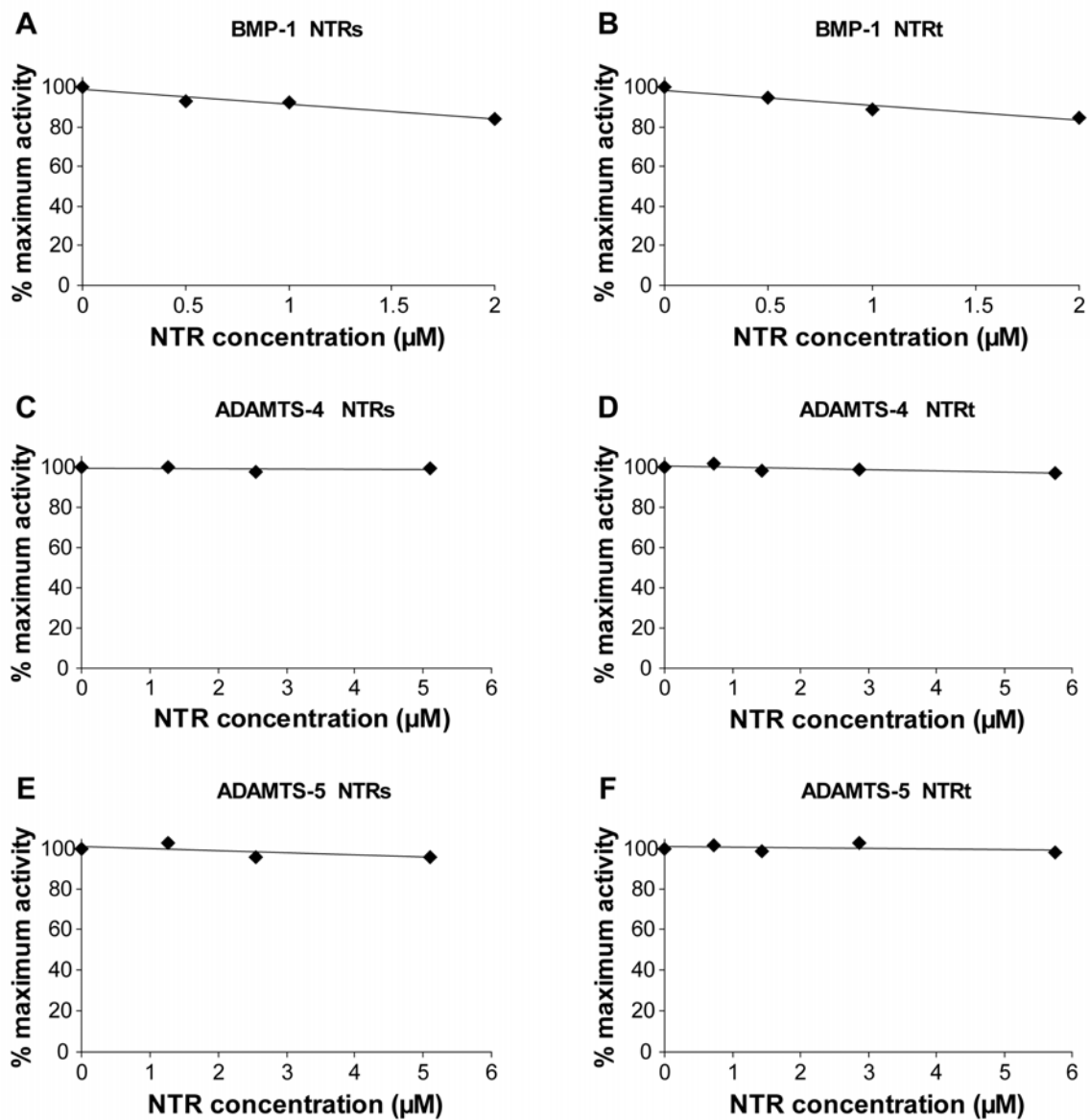
Supplemental Figure 2. Effects of NTRs and NTRt on the activities of (A,B) BMP-1, (C,D) ADAMTS-4 and (E,F) ADAMTS-5 using quenched fluorescent substrates (see Experimental Procedures).
