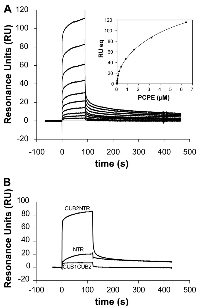
FIGURE 4. Binding of PCPE-1 to BMP-1 studied by surface plasmon resonance (Biacore). A, concentration dependence of binding of full-length PCPE-1 (12.5, 25, 50, 100, 200, 400, 800, 1600, 3200, and 6400 nM) to immobilized BMP-1 (500 RU). Inset , fit of the response at infinite time ( RU eq ) as a function of PCPE-1 concentration using the equation given under "Experimental Procedures." B, interactions of PCPE-1 fragments CUB1CUB2, NTRt, and CUB2-NTR (all at 500 nm) with immobilized BMP-1 (1463 RU).
