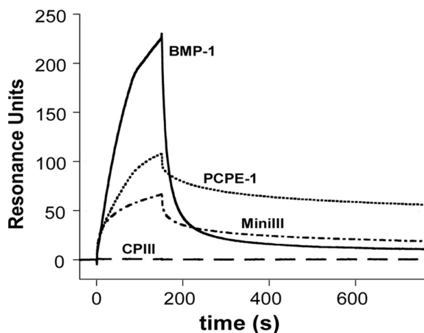
FIGURE 7. Interaction of PCPE-1, mini-procollagen III ( minIII ), the procollagen III C-propeptide trimer ( CPIII ), and BMP-1 with heparin. Biotinylated heparin was first bound to immobilized streptavidin to reach 44 RU and then solutions containing 50 nM of each protein were injected in 10 mM HEPES, 0.15 M NaCl, 0.05% P20 for 150 s at 30 µl/min.
