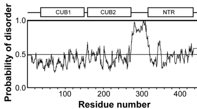
Supplemental Figure 3. The linker region between the CUB2 and NTR domains is intrinsically disordered. Prediction of intrinsically disordered regions using the program RONN (40).
