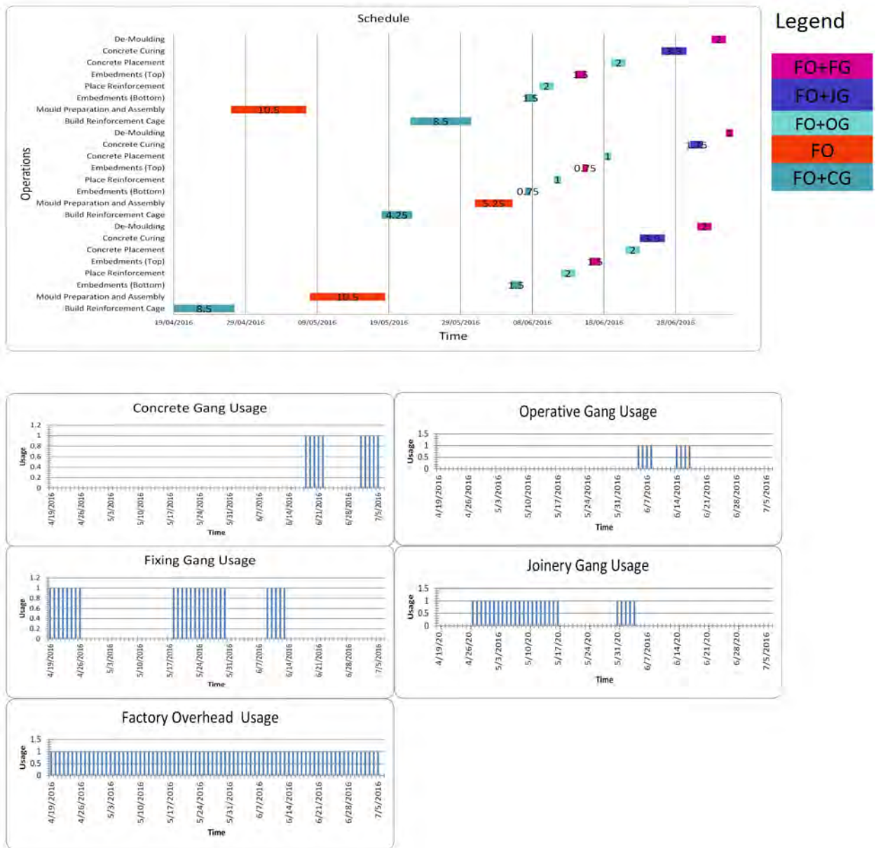
FIGURE 9 : Schedule obtained for the Manufacturing Line in TABLE 1 using the Proposed GA-based Algorithm
