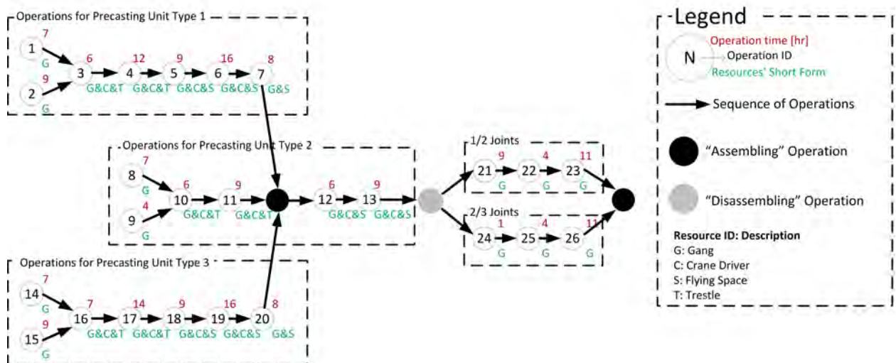
FIGURE 3 : A Representation of Operation Dependencies in a Unified MtA System
