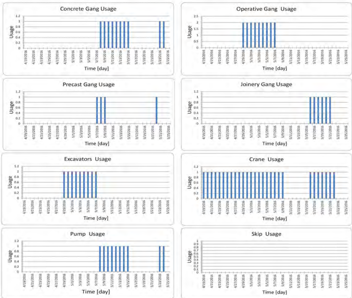
20 FIGURE 10 : Schedule obtained for the Assembly Line in TABLE 2 using the Proposed GA-based Algorithm
