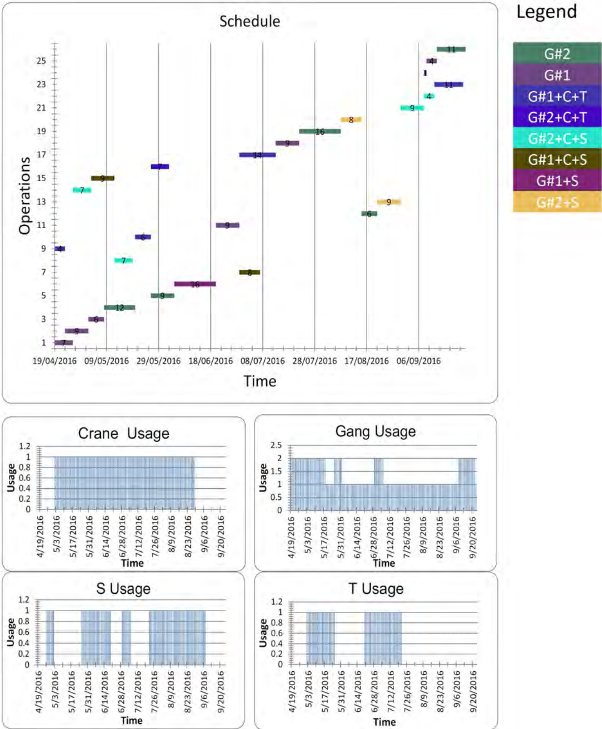
FIGURE 11 : Schedule obtained for the Conceptual Exercise of a Unified MtA System in FIGURE 3 using the Proposed GA-based Algorithm
