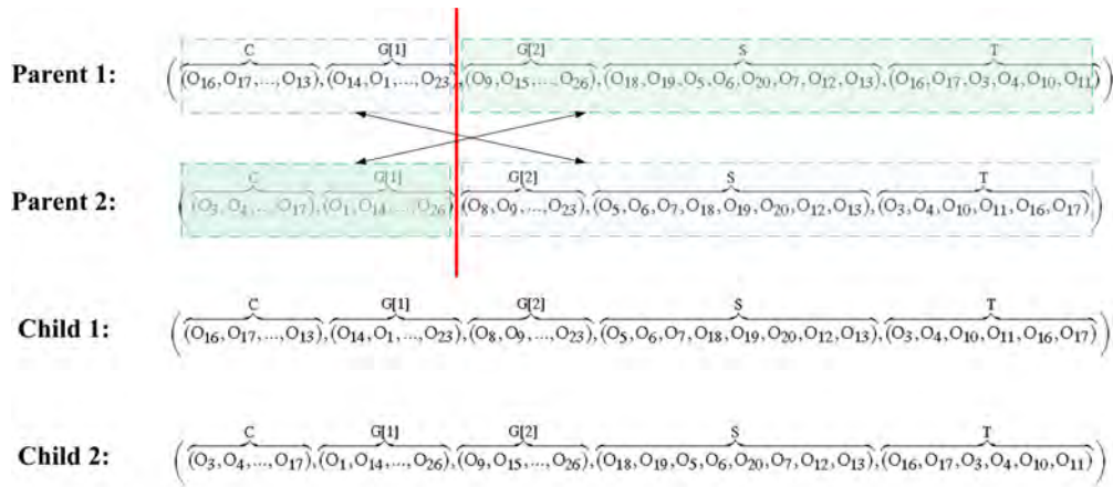
FIGURE 7 : Crossover Operator
