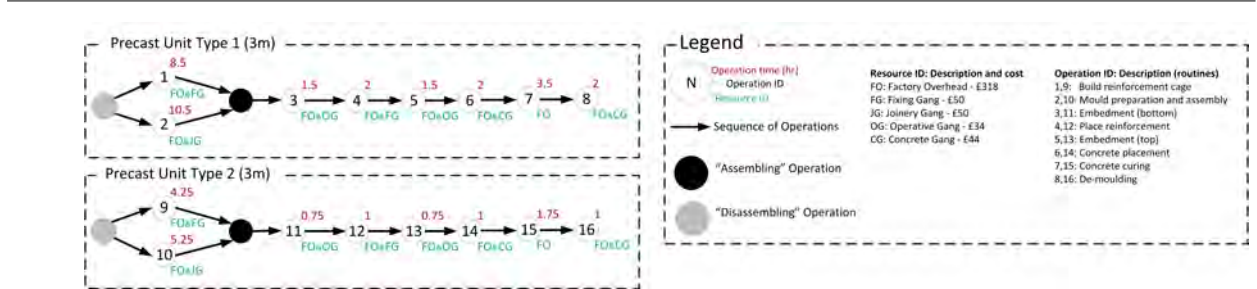
Operation Dependencies for Manufacturing Two Type of Precast Units
