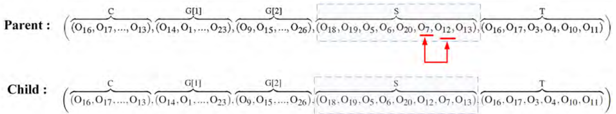
FIGURE 8 : Mutation Operator
