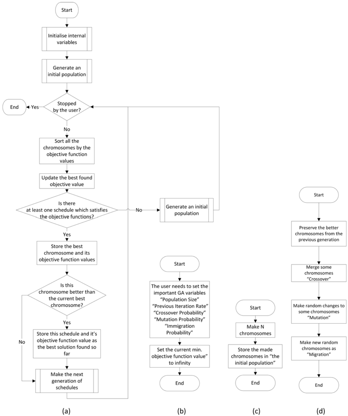
FIGURE 6 : The GA Assignment and Sequencing Procedures: (a) Overall Algorithm, (b) Parameter Initialisation, (c) Generating the Initial Population and (d) Sub-Sequential Iteration Algorithm
