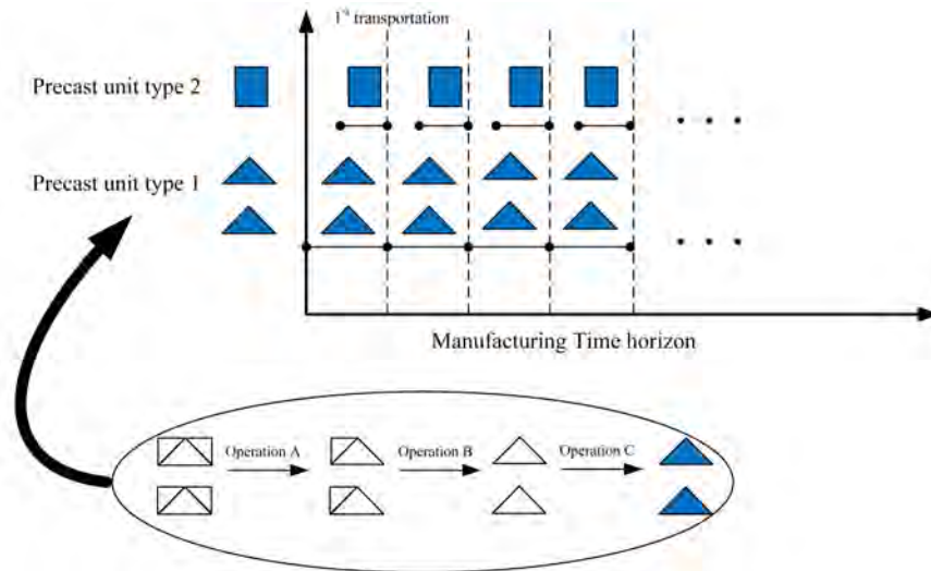
FIGURE 2 : An Example of Cyclic Jobs in a Manufacturing Line
