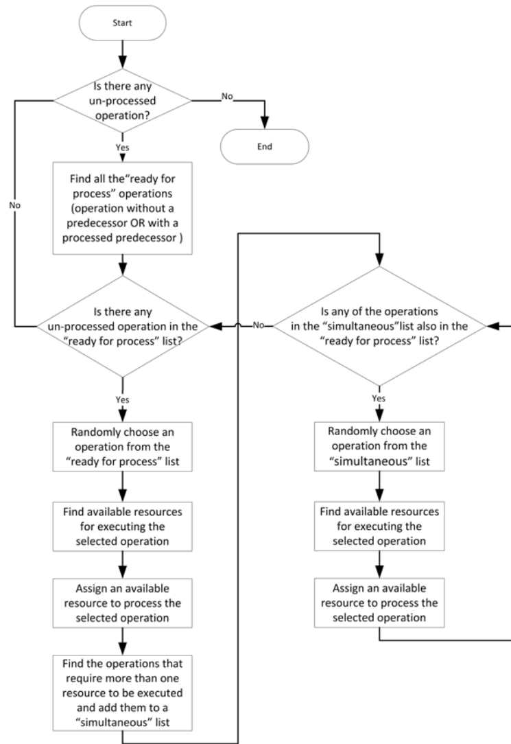
FIGURE 5 : Chromosome Encoding Procedure
