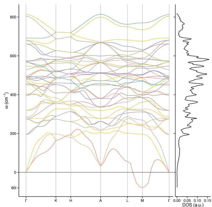
Figure 4 Dispersion curve and DOS for the hexagonal P6/mmm sub-cell of Ti 12 Be.
