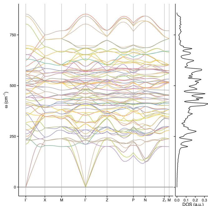
Figure 3 Dispersion curve and DOS of the tetragonal I4/mmm TiBe_{12} structure.
