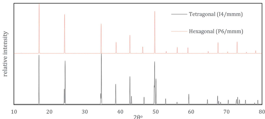
Figure 2 Simulated diffraction patterns for the fully ordered P6/mmm and I4/mmm unit cells.
