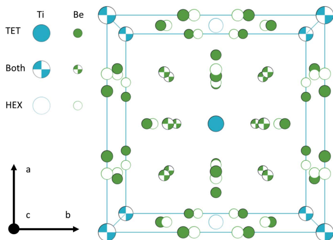
Figure 1 Correspondence between the I4/mmm tetragonal structure and the P6/mmm sub-cell for TiBe_{12} . In I4/mmm the a direction corresponds to the c direction in P6/mmm . Alternate Ti atoms are displaced by \frac{1}{2} in the I4/mmm [100] direction/ P6/mmm [0001] direction. Be positions are only slightly perturbed.
