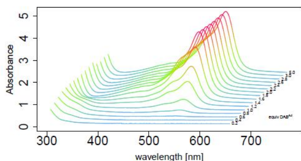
Figure 13. UV-vis spectra for the titration experiments with [\text{Cu}(\text{NCMe})_4]\text{BF}_4 (300 \mu\text{M} ) and different equivalents of \text{DAB}^{\text{Ad}} in DCM.
