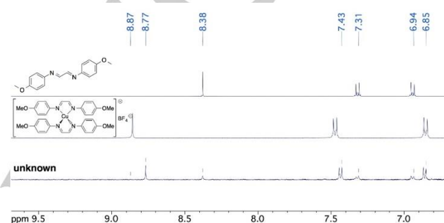
Figure 11. Comparison of ^1\text{H} NMR for the \text{Cu}/\text{DAB}^{\text{Anis}} system in \text{CD}_2\text{Cl}_2 .
