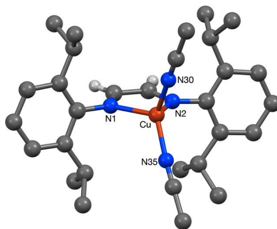
Figure 5. The structure of the cation present in the crystal of 5 . Most hydrogen atoms are omitted for clarity. Selected bond lengths (Å) and angles (°); Cu–N(1) 2.0821(12), Cu–N(2) 2.0798(12), Cu–N(30) 1.9424(15), Cu–N(35) 1.9391(14), N(1)–Cu–N(2) 78.82(5), N(1)–Cu–N(30) 112.60(6), N(1)–Cu–N(35) 117.91(5), N(2)–Cu–N(30) 110.21(6), N(2)–Cu–N(35) 117.88(5), N(30)–Cu–N(35) 114.52(6).
