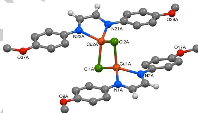
Figure 6. The structure of one (6-A) of the four independent complexes present in the crystal of [\text{CuCl}(\text{DAB}^{\text{Anis}})] 6 . Most hydrogen atoms are omitted for clarity.
