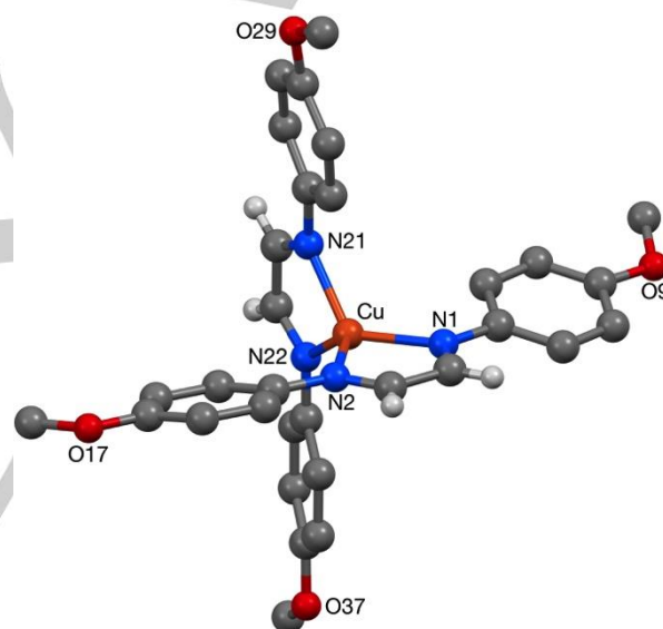
Figure 2. The structure of the cation present in the crystal of [\text{Cu}(\text{DAB}^{\text{Anis}})_2]\text{BF}_4 2 . Most hydrogen atoms are omitted for clarity. Selected bond lengths (Å) and angles ( ^\circ ); Cu–N(1) 2.0099(17), Cu–N(2) 2.0095(17), Cu–N(21) 2.0292(18), Cu–N(22) 2.0027(17), N(1)–Cu–N(2) 82.35(7), N(1)–Cu–N(21) 121.46(7), N(1)–Cu–N(22) 126.91(7), N(2)–Cu–N(21) 120.85(7), N(2)–Cu–N(22) 128.18(7), N(21)–Cu–N(22) 82.53(7), N(22) 145.46(7), N(2)–Cu–N(21) 145.49(7), N(2)–Cu–N(22) 107.64(7), N(21)–Cu–N(22) 82.41(6).
