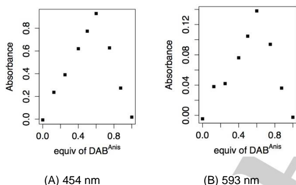
Figure 9. Jobs plot for the titration experiments with \text{DAB}^{\text{Anis}} in DCM.
