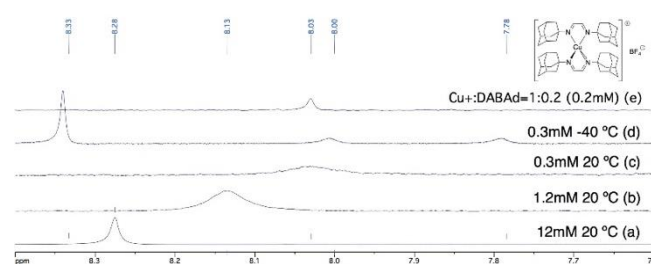
Figure 16. Comparison of 1 H NMR for the Cu/DAB Ad system in CD 3 CN.
