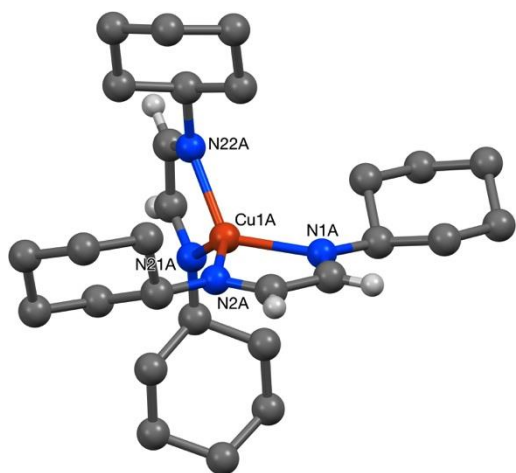
Figure 3. The structure of one (3-A) of the four independent cations present in the crystal of [\text{Cu}(\text{DAB}^{\text{Dy}})]_2\text{BF}_4 3 . Most hydrogen atoms are omitted for clarity.
