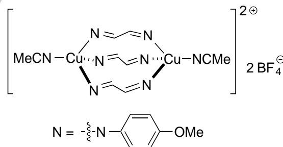
Figure 12. Plausible structure for the species formed by the \text{Cu}/\text{DAB}^{\text{Anis}} system in DCM.
