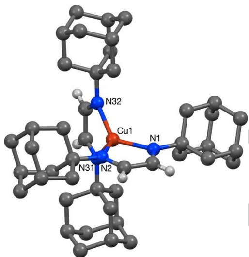
Figure 4. The structure of the cation present in the crystal of [\text{Cu}(\text{DAB}^{\text{Ad}})]_2\text{BF}_4 4 . Most hydrogen atoms are omitted for clarity. Selected bond lengths (Å) and angles (°); Cu(1)–N(1) 2.0374(11), Cu(1)–N(2) 2.0389(11), Cu(1)–N(31) 2.0559(12), Cu(1)–N(32) 2.0267(11), N(1)–Cu(1)–N(2) 81.95(5), N(1)–Cu(1)–N(31) 120.12(5), N(1)–Cu(1)–N(32) 129.81(5), N(2)–Cu(1)–N(31) 119.50(5), N(2)–Cu(1)–N(32) 128.66(5), N(31)–Cu(1)–N(32) 81.91(5).
