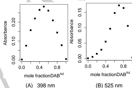
Figure 15. Jobs plot for the titration experiments with \text{DAB}^{\text{Ad}} in MeCN.
