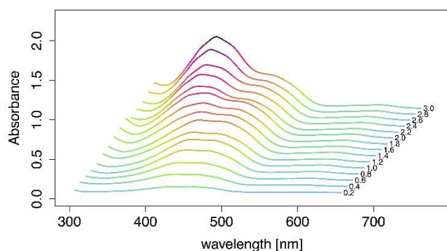
Figure 8. UV-vis spectra for the titration experiments with [\text{Cu}(\text{NCMe})_4]\text{BF}_4 ( 15 \mu\text{M} ) and different equivalents of \text{DAB}^{\text{Anis}} in DCM.
