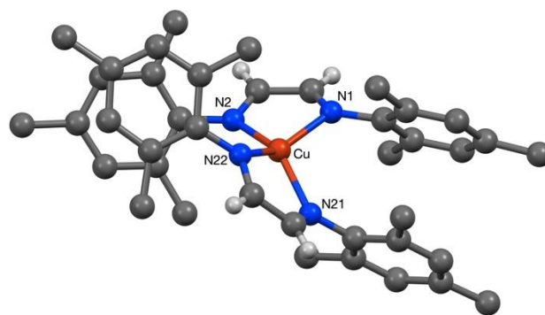
Figure 1. The structure of the cation present in the crystal of [\text{Cu}(\text{DAB}^{\text{Mes}})_2]\text{BF}_4 1 . Most hydrogen atoms are omitted for clarity. Selected bond lengths (Å) and angles ( ^\circ ); Cu–N(1) 2.0239(16), Cu–N(2) 2.0256(17), Cu–N(21) 2.0268(15), Cu–N(22) 2.0334(17), N(1)–Cu–N(2) 82.24(7), N(1)–Cu–N(21) 108.44(7), N(1)–Cu–N(22) 145.46(7), N(2)–Cu–N(21) 145.49(7), N(2)–Cu–N(22) 107.64(7), N(21)–Cu–N(22) 82.41(6).
