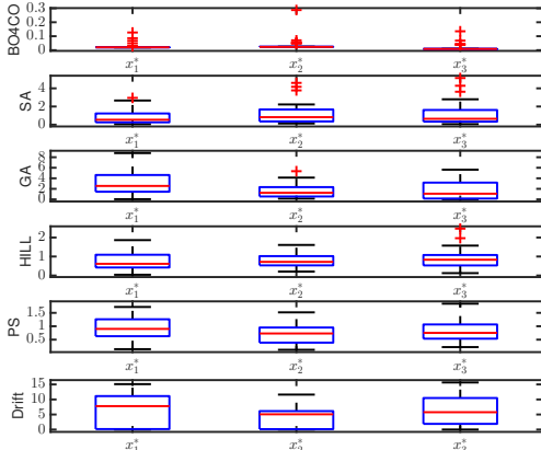
Fig. 11: Distance to the three Branin's minimizers.
