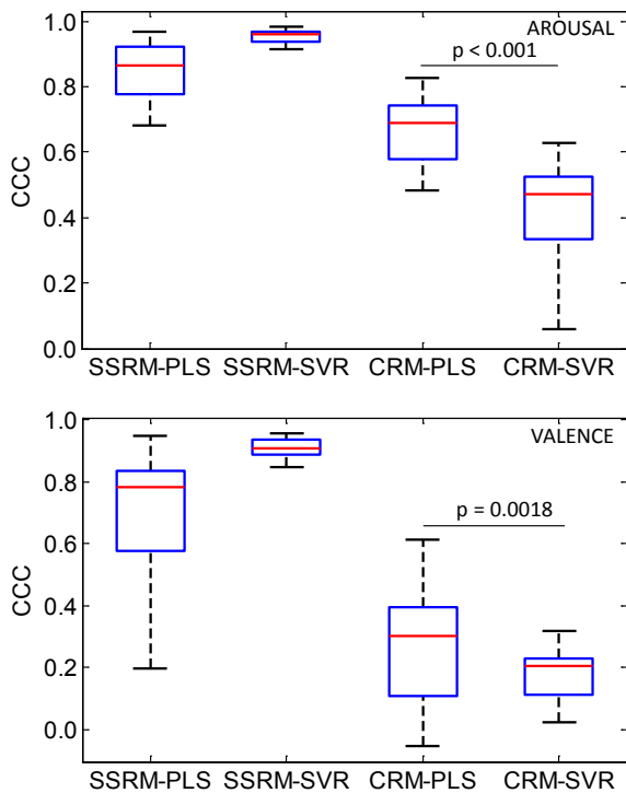
Fig. 11. Box-plots of the CCC values for the CRM applied using PLS regression compared with the CRM based on SVR. First and second column report the CCC values obtained during subject-dependent validation of each SSRM (SSRM-PLS and SSRM-SVR), third and fourth column indicate the CCC values during testing (CRM-PLS and CRM-SVR): p-values obtained by running paired t-test on the CCC values obtained for the CRM-PLS and the CRM-SVR are also indicated. Results are presented separately for arousal (top) and valence (bottom).
