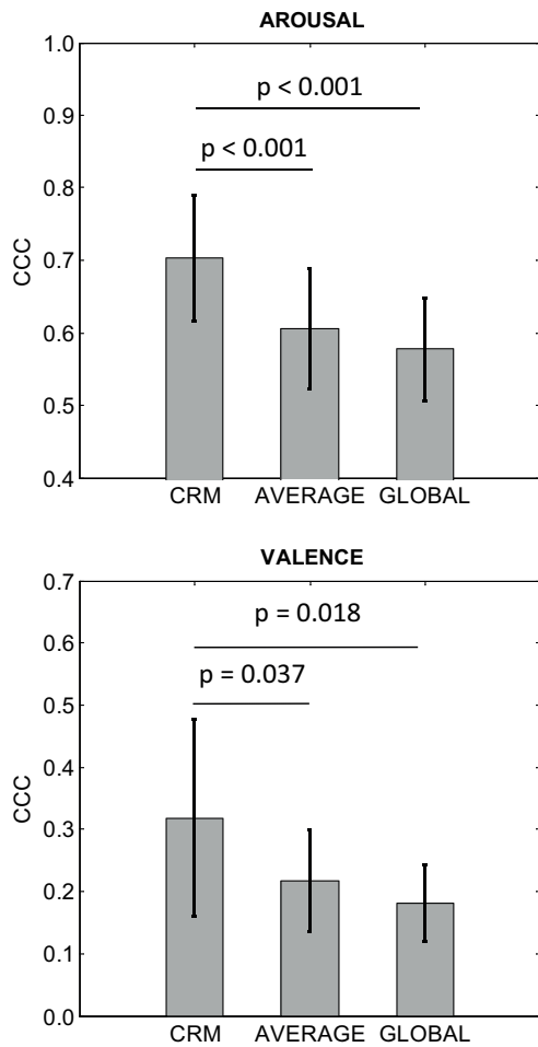
Fig. 7. Comparison of the performance (median and inter-quartile range of CCC) obtained with the proposed CRM, the average of all SSRM (AVERAGE) and a single PLS model learned on all the training data (GLOBAL) for arousal (top) and valence (bottom). The p-values obtained by a t-test on the CCC values between CRM and the two other methods are also indicated.
