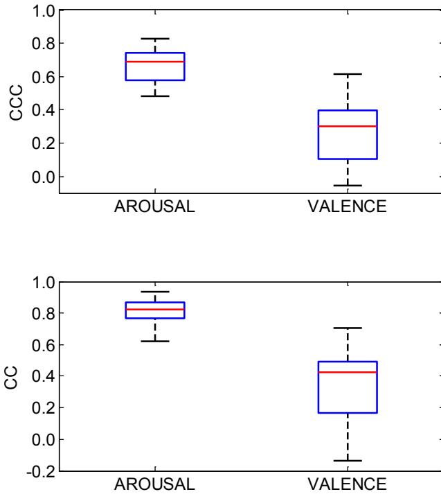
Fig. 5. Box-plots of CCC and CC values of the cooperative regression model applied to each speaker in testing phase for arousal and valence.
