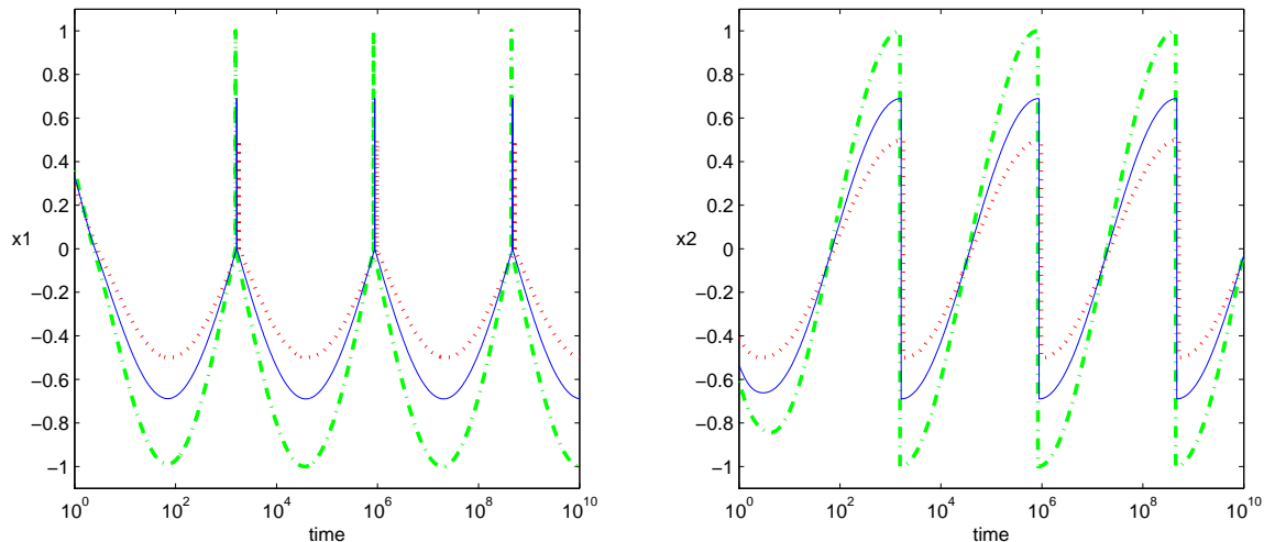
Fig. 2. Time histories of the states of the system (42) with p = 2 , q = 3 , k_1 = k_2 = 1 , \Psi(s) = |s| and x(0) = [0.5 \ 0 \ 1]' : \eta = 0 (red/dotted); \eta = 1 and r = 4 (blue/solid); \eta = 1 and r = 2 (green/dashed).
