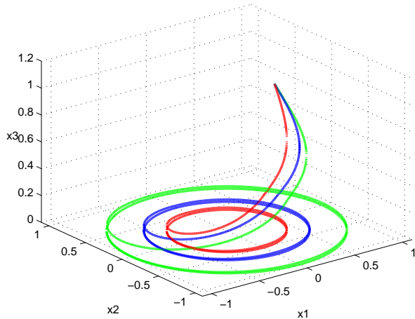
Fig. 1. The trajectory of system (42), with p = 2 , q = 3 , k_1 = k_2 = 1 , \Psi(s) = |s| , x(0) = [0.5 \ 0 \ 1]' , for the three considered cases. The trajectory converges to the circle of radius \rho_0 = 0.5 for \eta = 0 (red/dotted); of radius \min(1, \rho_0) \leq \rho \leq \max(1, \rho_0) for \eta = 1 and r = 4 (blue/solid); of radius 1 for \eta = 1 and r = 2 (green/dashed).
