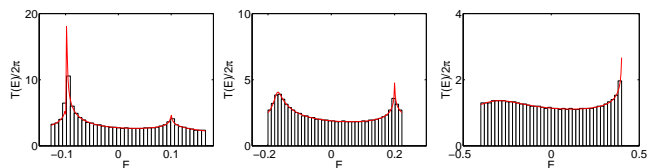
FIG. 13: (Color online) (m, n) = (3, 2) : Mean-field period T(E) divided by 2\pi (red line) and many-particle density of states (histogram) for N = 9000 particles for v = 1 and \epsilon = 0.2, 0.4, 0.8 from left to right.
