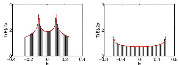
FIG. 10: (Color online) (m, n) = (2, 2) : Mean-field period T(E) divided by 2\pi (red line) and many-particle density of states (histogram) for N = 9000 particles for v = 1 and \epsilon = 0.2 (left) and \epsilon = 1.2 (right).
