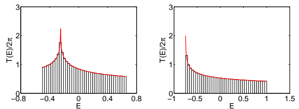
FIG. 9: (Color online) (m, n) = (2, 1) : Mean-field period T(E) divided by 2\pi (red line) and many-particle density of states (histogram) for N = 9000 particles for v = 1 and \epsilon = 0.5 (left) and \epsilon = 1.5 (right).
