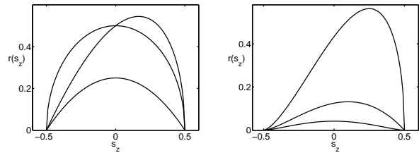
FIG. 2: Radius r(s_z) of the Kummer surface (45) for (m, n) = (1, 1), (2, 1), (2, 2) (left) and (3, 1), (3, 2), (3, 3) (right).
