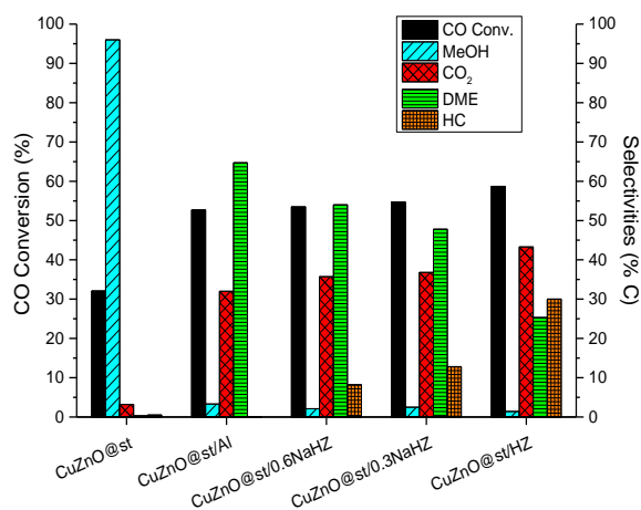
Fig. 3. CO conversions and selectivities for CuZnO@st/ \gamma Al hybrid catalysts prepared with a CuZnO/ x mass ratio of 1/1. Reaction conditions: 260 °C, 5.0 MPa, GHSV = 7.4 L syn-gas /g CuZn /h and syn-gas composition 70%H 2 /24%CO/6%CO 2 .
