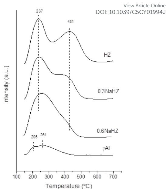
Fig. 2. NH 3 -TPD profiles for the HZ, NaHZ and \gamma Al acid samples.
