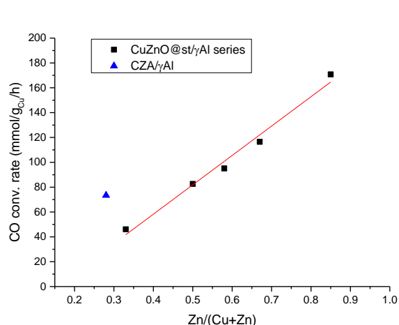
Fig. 5. CO conversion rate (per mass of copper) as a function of Zn content for the CuZnO@st/γAl and the reference CZA/γAl hybrid catalysts.
