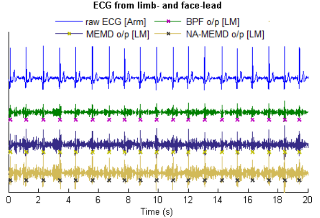
Fig. 3: Signal and detected peaks (crosses) after applying the methods BPF, MEMD, and NA-MEMD to measurements at the LM collated with limb-lead ECG.
