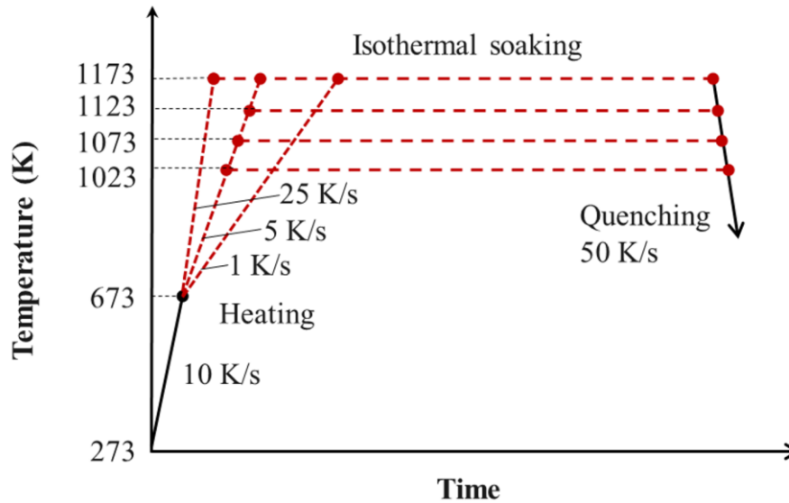
Figure 2 Testing programme with different heating rates (first group) and soaking temperatures (second group).
