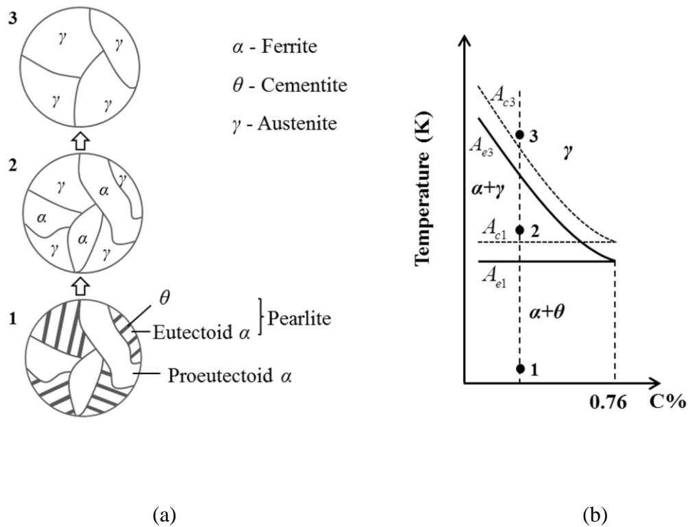
Figure 1 The formation of austenite in a hypoeutectoid steel (containing less than 0.76wt% C), illustrated by (a) the schematic representations of the microstructure and (b) the evolution in a Fe-C phase diagram (only hypoeutectoid part).
