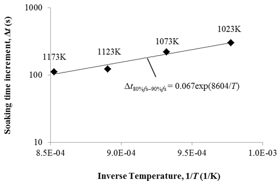
Figure 11 Effect of soaking temperature on the transformation time to increase austenite volume fraction by 10% of f_s from 80% of f_s .
