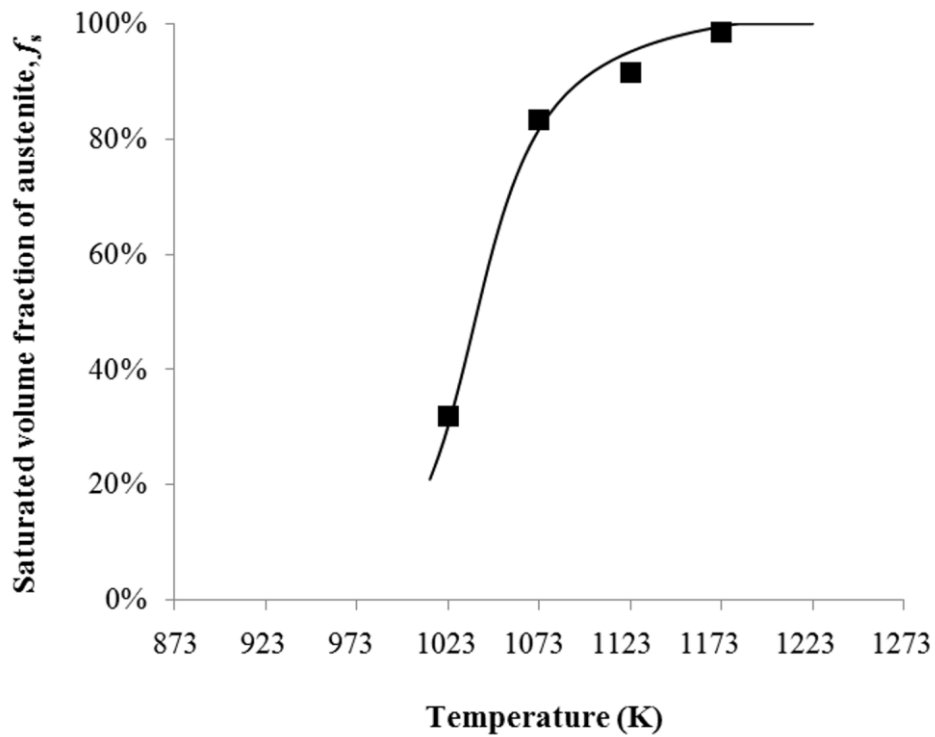
Figure 10 Saturated volume fractions of austenite at different soaking temperatures.
