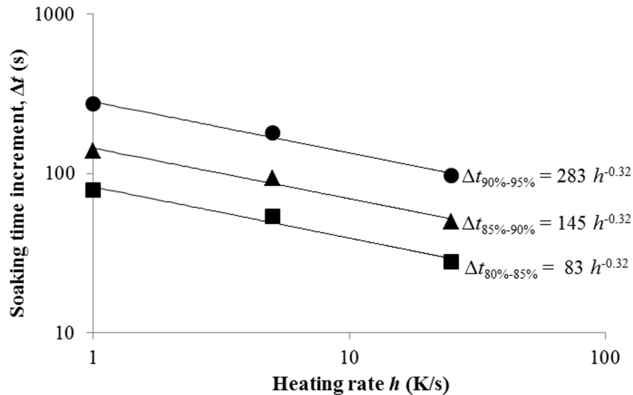
Figure 8 Effect of heating rate on the transformation time to increase austenite volume fraction by 5% from 80%, 85% and 90% during soaking at 1173K.
