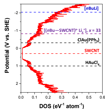
Fig. 4 The averaged DOS of the ( n,m ) distribution in a HiPco sample was derived from ref. 13. 22 The averaged DOS comprises 28 semi-conducting and 18 metallic SWCNTs as identified from resonance Raman spectroscopy. 23 For simplicity, all ( n,m )-SWCNTs equally contribute to the DOS, although, as in a typical SWCNT sample the proportion of semi-conducting:metallic SWCNTs is adjusted to 2:1. The position of the Fermi level, E F , of undoped HiPco SWCNTs was determined from cyclic voltammetry (~+0.30 V vs. SHE), although in principle, the E F will vary for each ( n,m )-SWCNT. 1, 24
