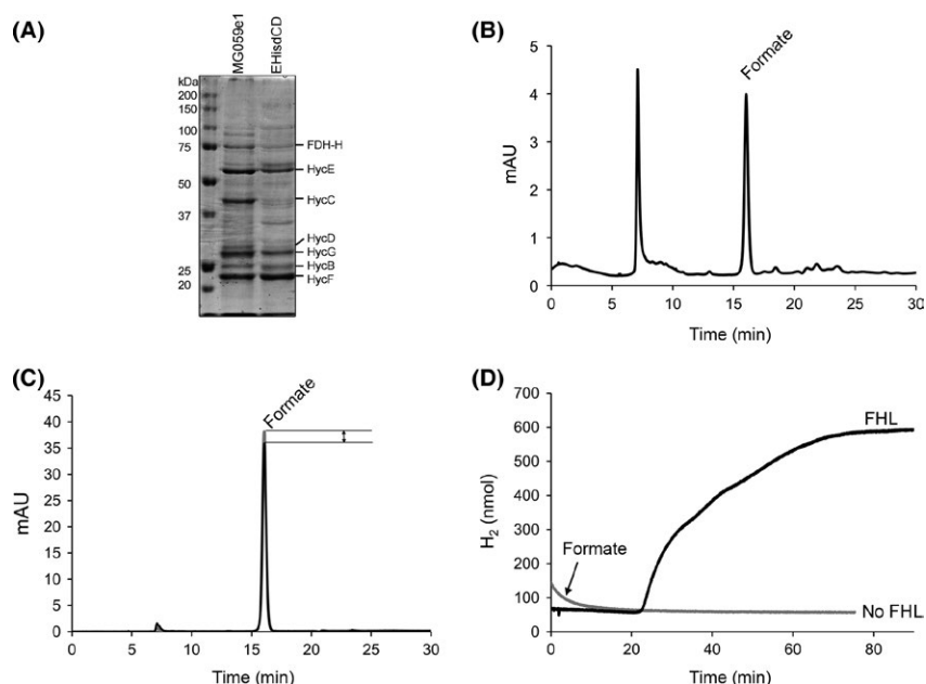
Figure 4. Reactions of purified formate hydrogenlyase (FHL-) complex in vitro. (A) Purified protein (30 \mu g) from strains MG059e1 (FHL with internal His-tag on HycE) and EHisdCD (same as MG059e1, but with deletion of hycCD ) was applied to a 10% (w/v acrylamide) SDS-PAGE and separated. The molecular mass of the ladder is given on the left-hand side (PageRuler Plus, Fisher Scientific). (B) A representative high-performance liquid chromatography (HPLC) profile of formate production by purified FHL complex (370 \mu g) after incubation under \text{CO}_2 and \text{H}_2 atmosphere for 5 h at 37°C. An aliquot of 10 \mu L was applied directly to an Aminex HPX 87H column at 50°C and separated compounds detected at A_{210 \text{ nm}} . The formate peak elutes at 16.2 min, whereas the injection peak can be seen at 7 min. (C) Representative HPLC analysis of formate content before (gray, 15.74 mmol/L from a stock solution) and after incubation with 370- \mu g purified FHL complex (approx. 1.2 nmol) for 5 h at 37°C (black trace, 14.90 \pm 0.07 mmol/L, n = 5 , P < 0.01 using a paired t -test). (D) A representative assay of the forward reaction using detergent-solubilized, purified FHL (370 \mu g) in a hydrogen-sensing Clark-type electrode. The trace (black) shows the reaction when initiated through the addition of 15 mmol/L (final concentration) formate. Strict anaerobiosis is required for this assay and this reaction was therefore carried out in the presence of an enzymatic oxygen scavenger system with D-glucose, glucose oxidase, and catalase as described (Sargent et al. 1999). The lag time before the reaction commences is considered to be due to the time taken to reduce residual \text{O}_2 in the reaction vessel to noninhibitory levels. The same oxygen-scavenging components were added in the absence of FHL complex as a control (gray trace).
