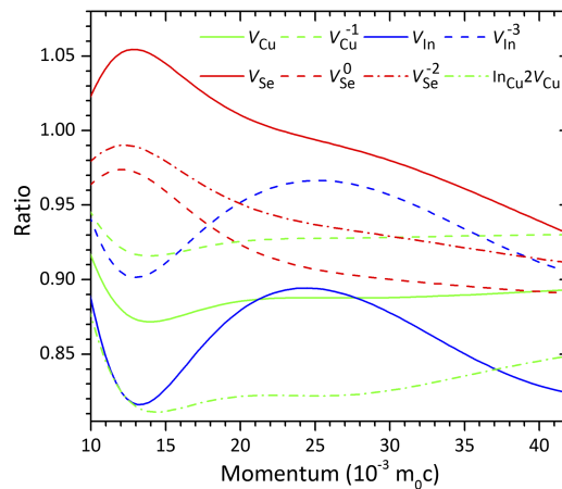
FIG. 3. Atomic superposition DFT calculated coincidence Doppler spectroscopy ratio spectra for various relaxed states of the monovacancy defects in \text{CuInSe}_2 . The spectra obtained using unrelaxed geometries for the defects; \text{In}_{\text{Cu}}2\text{V}_{\text{Cu}} is included for comparison.
