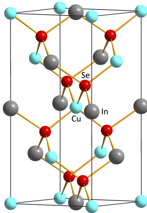
FIG. 1. Schematic of the ideal \text{CuInSe}_2 lattice.
