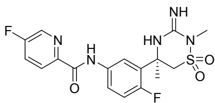
Figure 2. Chemical structure of BACE-1 inhibitor 5 .
