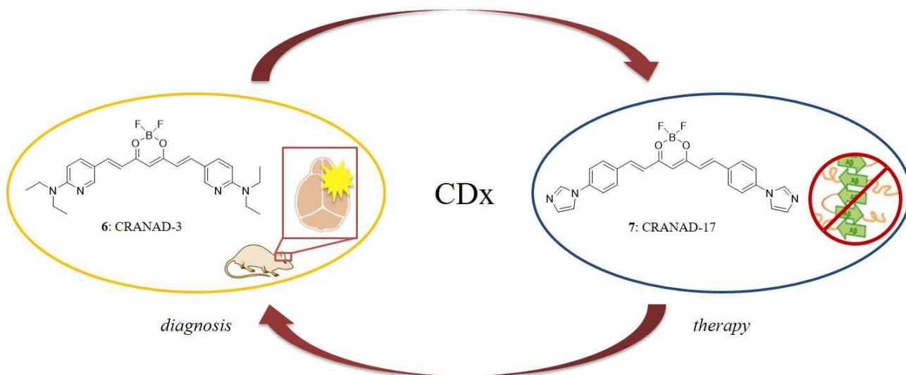
Figure 3. Development of the first fluorescent CDx validated in an AD mouse model.
