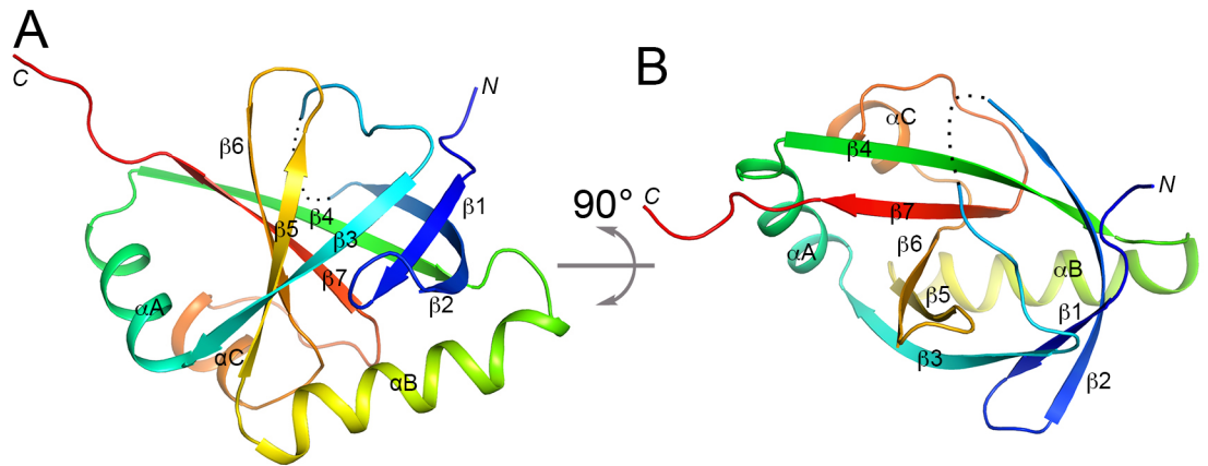
Fig 2. Crystal structure of the SPOC domain of A. thaliana FPA. (A). Schematic drawing of the structure of FPA SPOC domain, colored from blue at the N terminus to red at the C terminus. The view is from the side of the \beta -barrel. The disordered segment (residues 460–465) is indicated with the dotted line. (B). Structure of the FPA SPOC domain, viewed from the end of the \beta -barrel, after 90^\circ rotation around the horizontal axis from panel A. All structure figures were produced with PyMOL ( www.pymol.org ).
