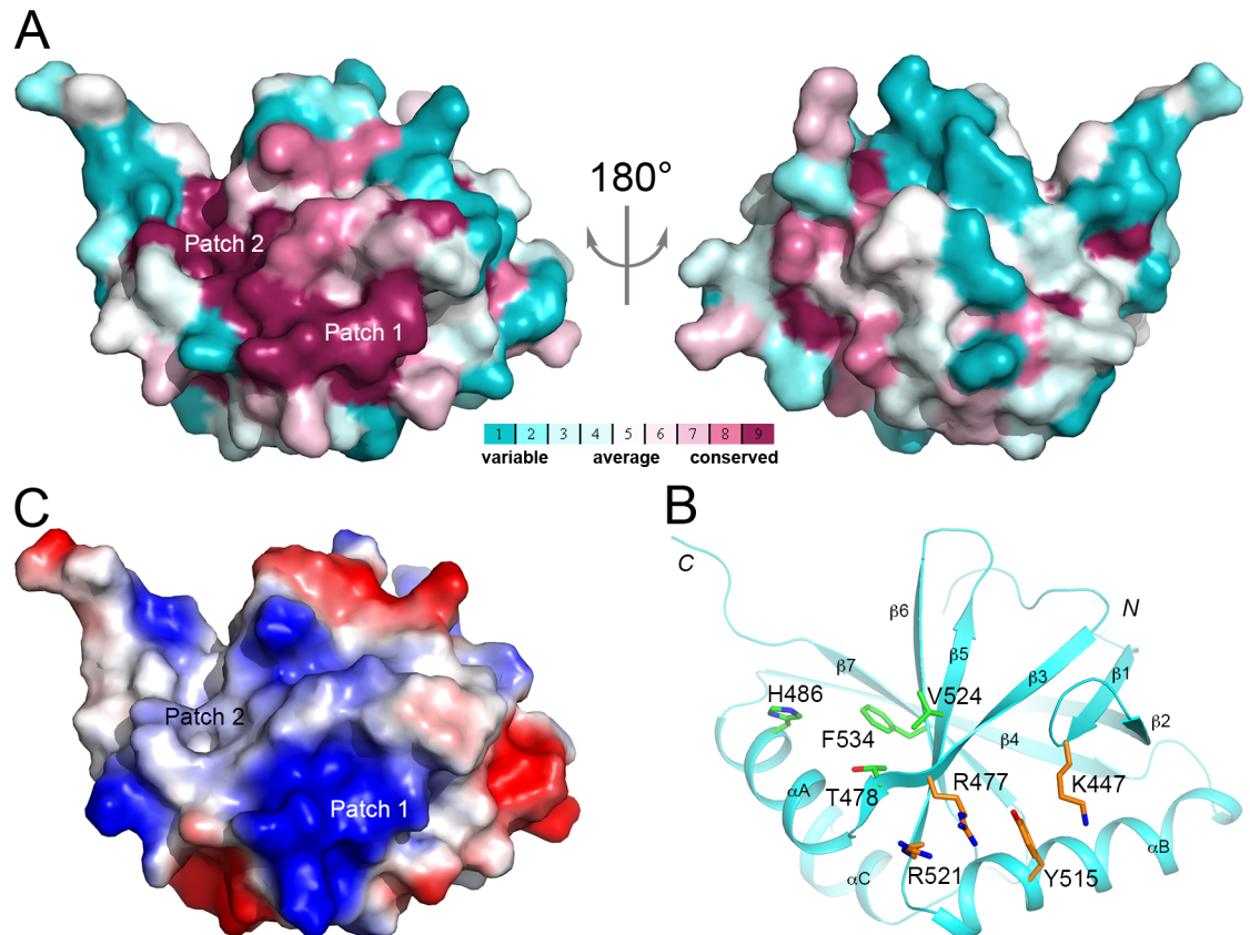
Fig 4. A conserved surface patch of FPA SPOC domain. (A). Two views of the molecular surface of FPA SPOC domain colored based on sequence conservation among plant FPA homologs. Purple: most conserved; cyan: least conserved. (B). Residues in the conserved surface patch of FPA SPOC domain. The side chains of the residues are shown in stick models, colored orange in the first sub-patch and green in the second. (C). Molecular surface of FPA SPOC domain colored based on electrostatic potential. Blue: positively charged; red: negatively charged.
