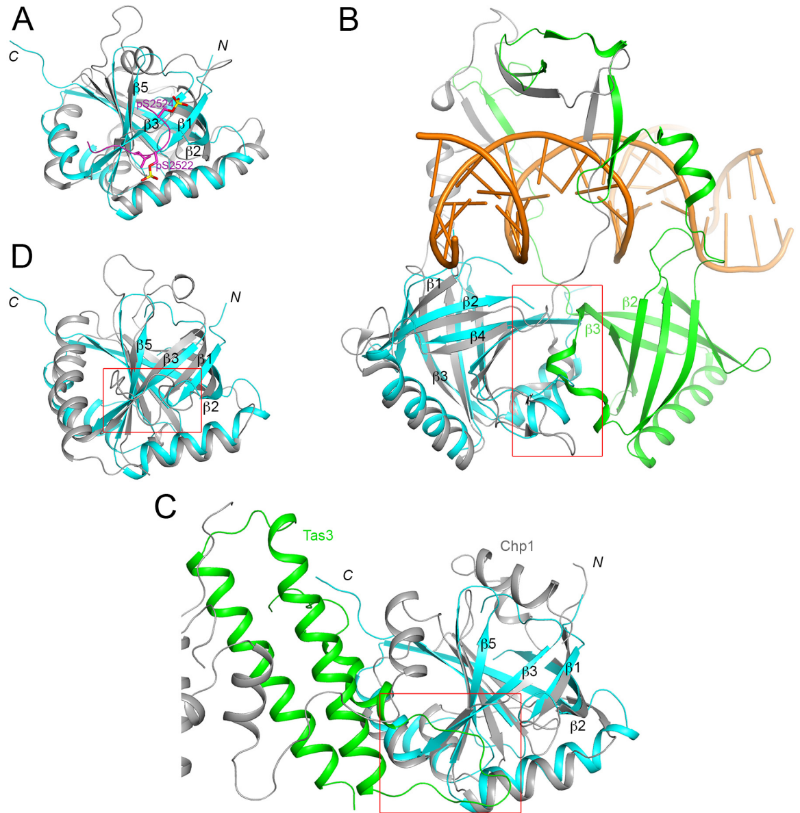
Fig 3. Structural homologs of the FPA SPOC domain. (A). Overlay of the structures of the FPA SPOC domain (cyan) and the SHARP SPOC domain (gray). The bound position of a doubly-phosphorylated peptide from SMRT is shown in magenta. (B). Overlay of the structures of the FPA SPOC domain (cyan) and the Ku70 \beta -barrel domain (gray). Ku80 contains a homologous domain (green), which forms a hetero-dimer with that in Ku70. The two domains, and inserted segments on them, mediate the binding of dsDNA (orange). The red rectangle highlights the region of contact between the two \beta -barrel domains. (C). Overlay of the structures of the FPA SPOC domain (cyan) and the homologous domain in Chp1 (gray). The binding partner of Chp1, Tas3, is shown in green. The red rectangle indicates the region equivalent to the binding site of the SMART phosphopeptide in SHARP SPOC domain, where a loop of Tas3 is also located. (D). Overlay of the structures of the FPA SPOC domain (cyan) and the Med25 ACID (gray).
