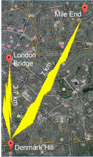
Fig. 2. The 7 km and 3.7 km long-distance links across London, that were have thus-far been tested in our trials.
