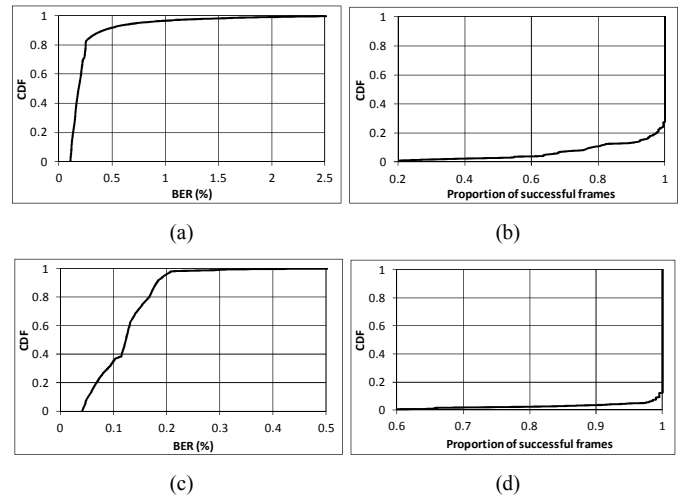
Fig. 4. Modulation and coding testing results for Link 1: (a) BER for 16-QAM with no coding, (b) frame success probability for 16-QAM with no coding, (c) BER for 16-QAM with \frac{1}{2} -rate convolutional coding, (d) frame success probability for 16-QAM with \frac{1}{2} -rate convolutional coding.
