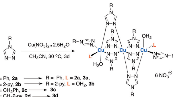
Scheme 1 Preparation of Cu-triazole complexes.
