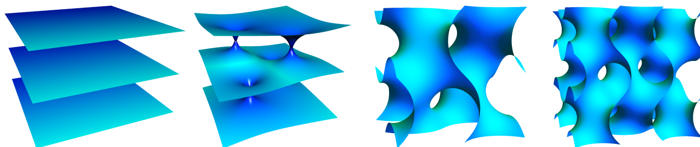
Figure 5: Summary of the proposed transition from a flat lamellar structure to inverse bicontinuous cubic gyroid phase. The figures shows the bilayer mid-plane in (from left to right): flat lamellar phase, uncorrelated inter-lamellar attachments (ILAs), swollen gyroid structure, equilibrium gyroid phase.
