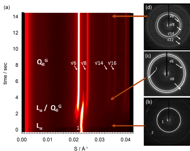
Figure 1: (a) Stacked diffraction plot showing the diffraction pattern during a lamellar to Q_{II}^G transition triggered by a pressure jump from P_{start} = 1800 bar to P_{end} = 440 bar with P_{amp} = -835 bar (where P_{amp} is defined as the pressure difference between the lamellar - lamellar / Q_{II}^G phase boundary and the end of the pressure jump ( P_{end} )). Typical 2d diffraction patterns from (b) the lamellar phase before the start of the jump, (c) lamellar and Q_{II}^G phase coexistence during the pressure jump (enlarged for clarity) and (d) and Q_{II}^G phase at the end of the pressure jump.
