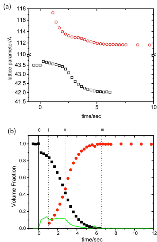
Figure 2: Structural changes of the lamellar and Q_{II}^G phase during a pressure jump ( P_{start} = 1800 bar, P_{end} = 440 bar, P_{amp} = -835 bar) starting in the lamellar phase, time = 0 denotes time of pressure jump. (a) Changes in lattice parameter of the outgoing lamellar phase (black open squares) and the incoming Q_{II}^G phase (red open circles); (b) change in the volume fraction of the lamellar phase (black closed squares), Q_{II}^G phase (red closed circles) and non-diffracting structural intermediate (green line).
