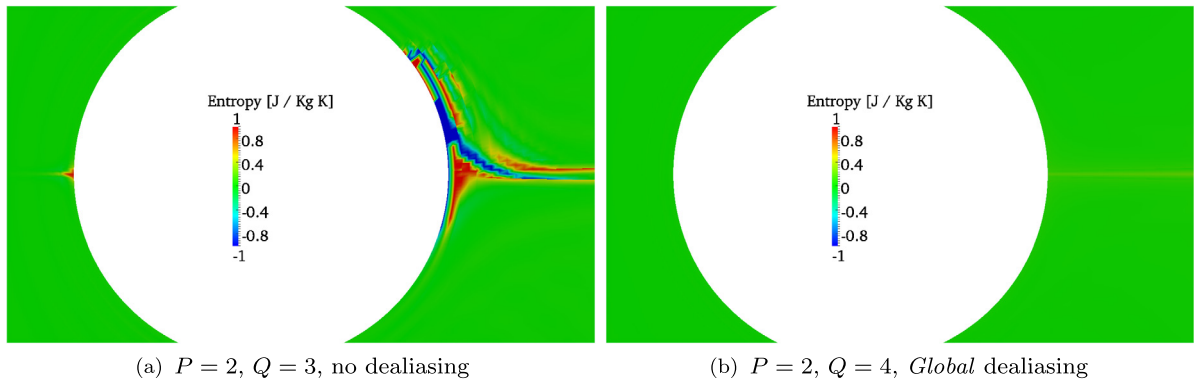
Fig. 13. Numerically-generated entropy for P = 2 .
