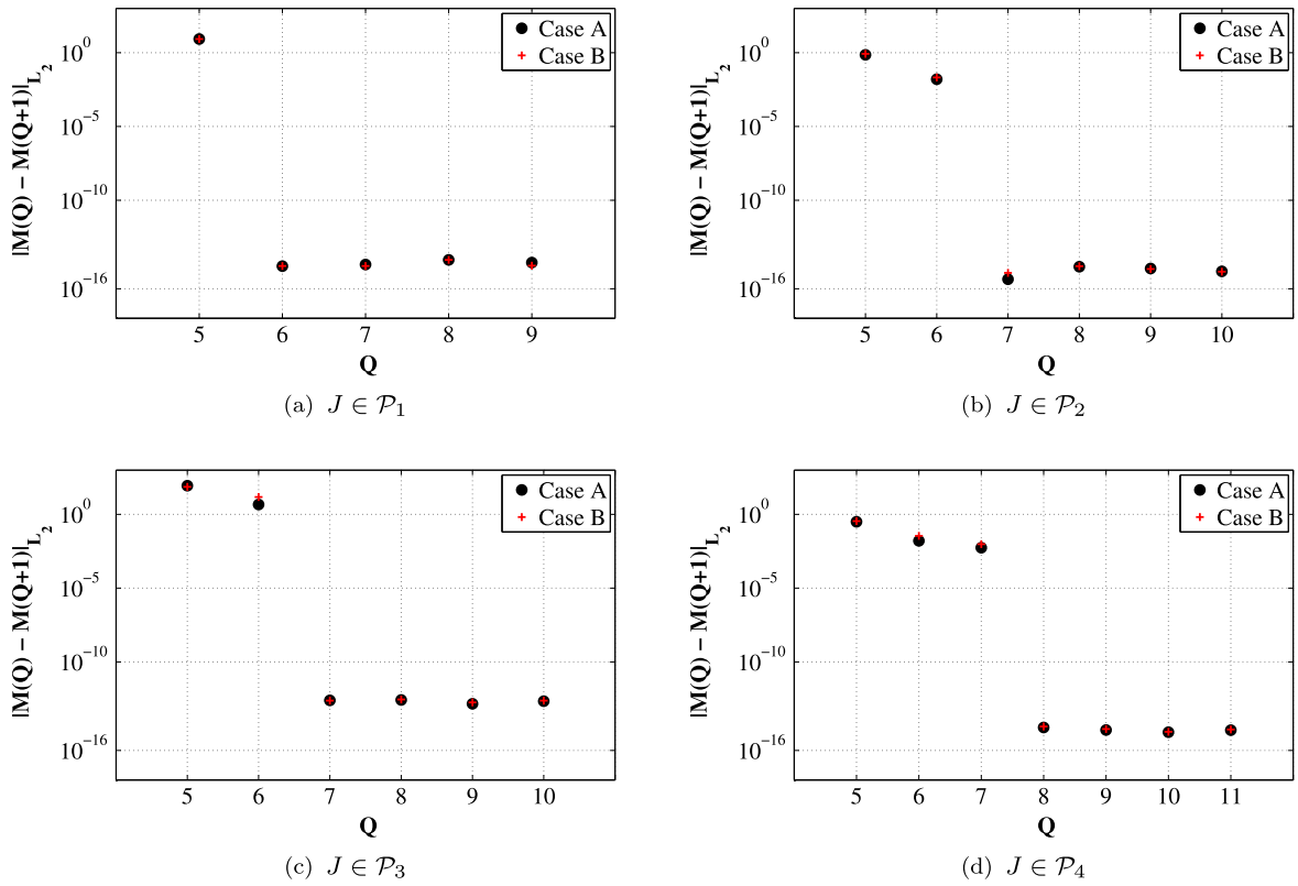
Fig. 10. L_2 norm of the difference between mass matrices calculated with Q and Q + 1 GLL points for the four orders considered and using both the mesh configurations shown in Fig. 8. Case A corresponds to Fig. 9(a) and Case B corresponds to Fig. 9(b).
