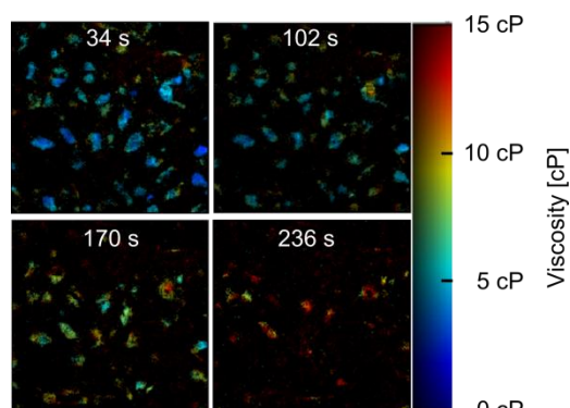
Figure 6. Viscosity maps obtained from ratiometric images of SK-OV-3 cells upon different irradiation times, shown in white above images; \lambda_{\text{exc}} = 453 nm.
