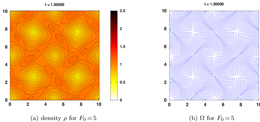
Figure 4.6: Solution of the SOHR model for F_0 = 5 . Density \rho (fig 4.6a ), flux direction \Omega (fig.4.6b ) at t = 1.5s .
