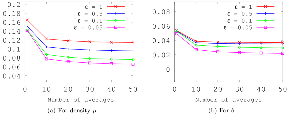
Figure 4.2: Relative error between the macroscopic and the microscopic model for density (a) and \theta (b) as a function of the number of averages for different values of \varepsilon . The error decreases with both decreasing \varepsilon and increasing number of averages, showing that the SOHR model provides a valid approximation of the IBM for \rho and \theta .
