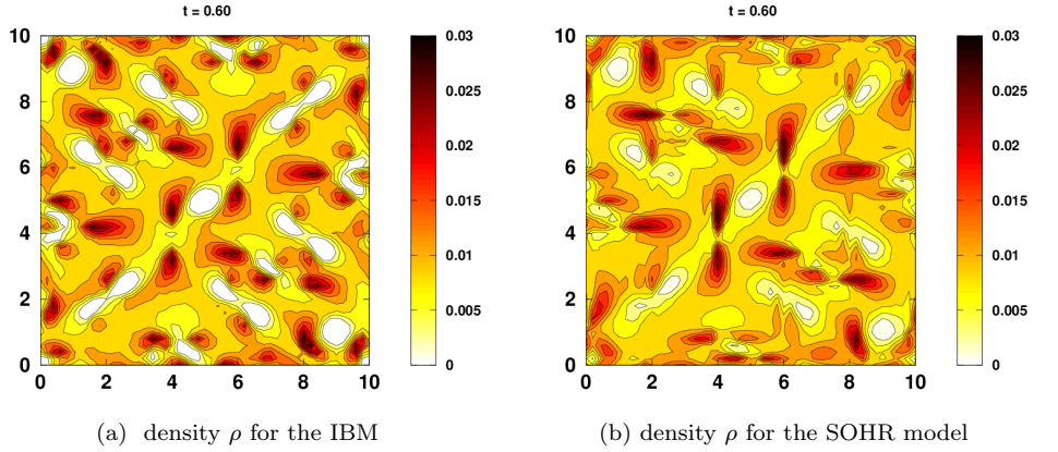
Figure 4.4: Density \rho for Taylor-Green vortex problem 4.4 at time t = 0.6s . Left: IBM. Right: SOHR model.
