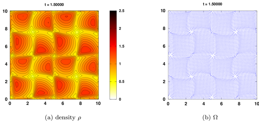
Figure 4.8: Solution of the DLMP model for F_0 = 5 . Density \rho (left) and flux direction \Omega (right) at t = 1.5s .
