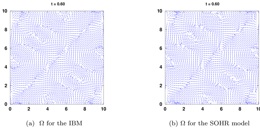
Figure 4.5: Mean direction \Omega for Taylor-Green vortex problem 4.4 at time t = 0.6s . Left: IBM. Right: SOHR model.
