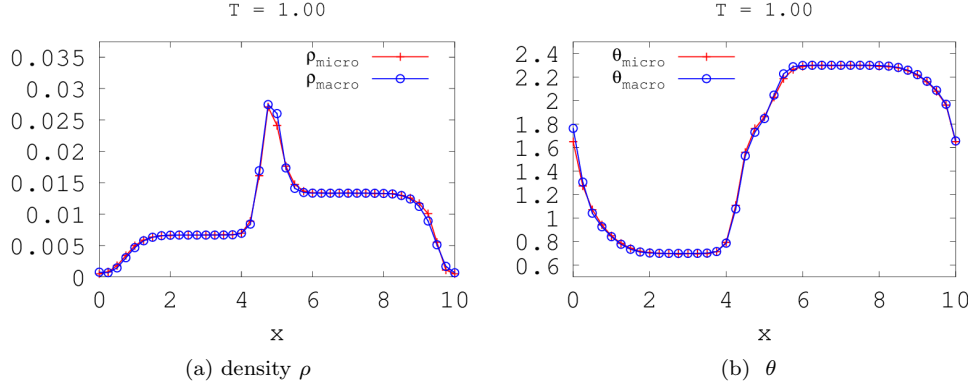
Figure 4.3: Solution of the Riemann problem (4.3) along the x -axis for the SOHR model (blue line) and for the IBM with \varepsilon=0.05 (red line) at T=1s . The agreement between the two models is excellent. For the SOHR model, the mesh size is \Delta x = \Delta y = 0.0625 .
