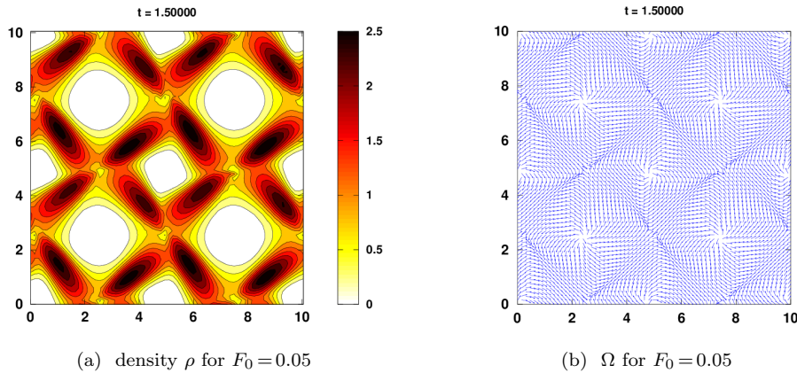
Figure 4.7: Solution of the SOHR model for F_0 = 0.05 . Density \rho (fig 4.6a ), flux direction \Omega (fig.4.6b ) at t = 1.5s .
