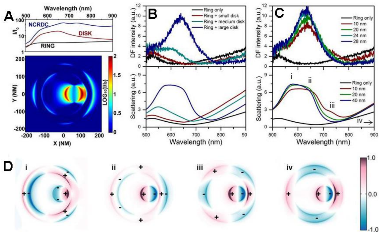
Figure 8. Non-concentric Ring-Disk Cavities for extending the spectral range of coupling.
