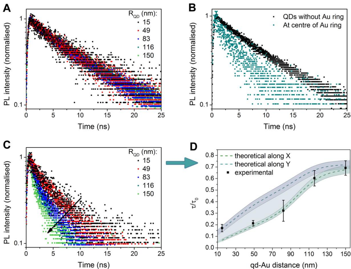
Figure 5. Radiative properties of QDs coupled to PRCs as a function of QD-Au separation.
