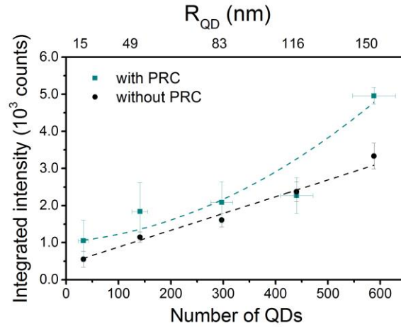
Figure 6. Integrated intensity of a rings of QD650 of various diameters, standalone (black scatter points) and coupled to a D440t60 PRC (green scatter points). The radius of the QD ring ( R_{QD} ) and the corresponding approximate number of QDs are indicated on the top and the bottom axis respectively. The standalone data follows a linear relationship (dashed black line). The green dashed line for coupled QDs is a visual guide only, but clearly shows the nonlinear relationship. In both cases, emission intensity was integrated over the entire time window during lifetime measurements (100 ns).
