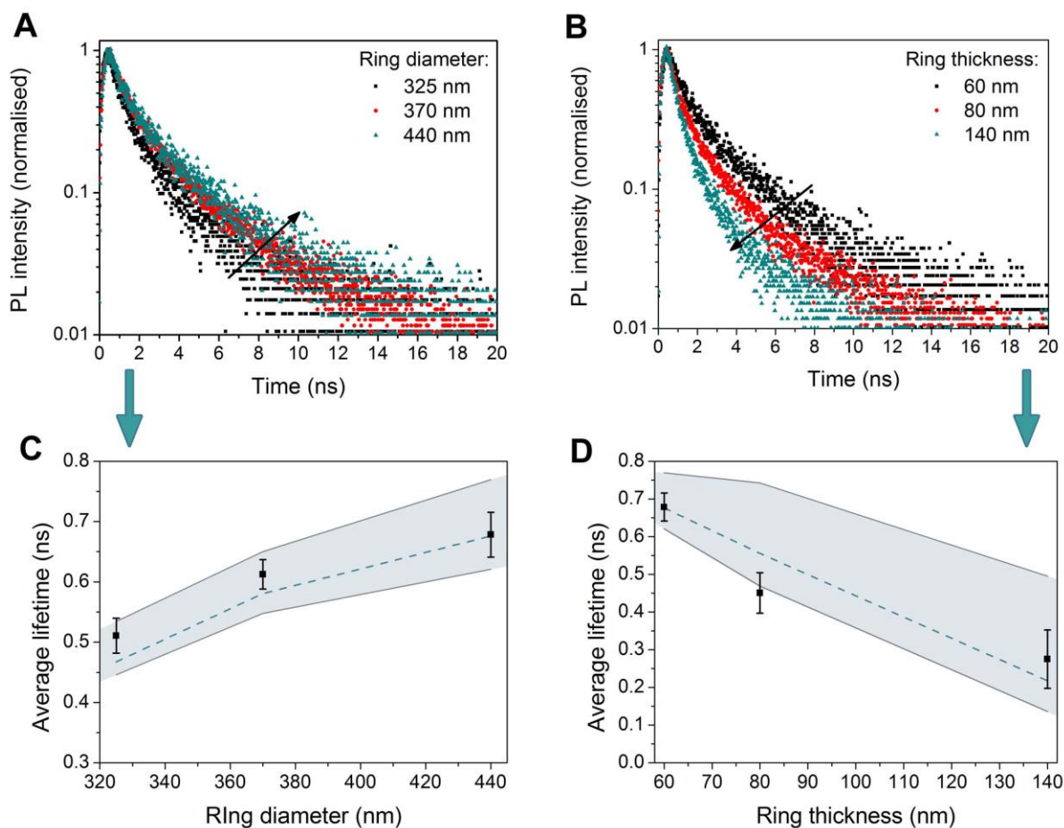
Figure 7. Radiative properties of QDs as a function of PRCs' dimensions. (A) and (C) show effect of increasing PRC's outer diameter on the fluorescence decay of QDs coupled to the PRC, while (B) and (D) show similar data for increasing thickness of the PRC. (A) and (B) are experimental fluorescence decay curves; while (C) and (D) show the average fluorescence lifetime values extracted from the experimental data (black scatter points), and the possible theoretical values of lifetimes (light blue bands) averaged over possible locations of QDs and the spread of their emission (dashed lines).
