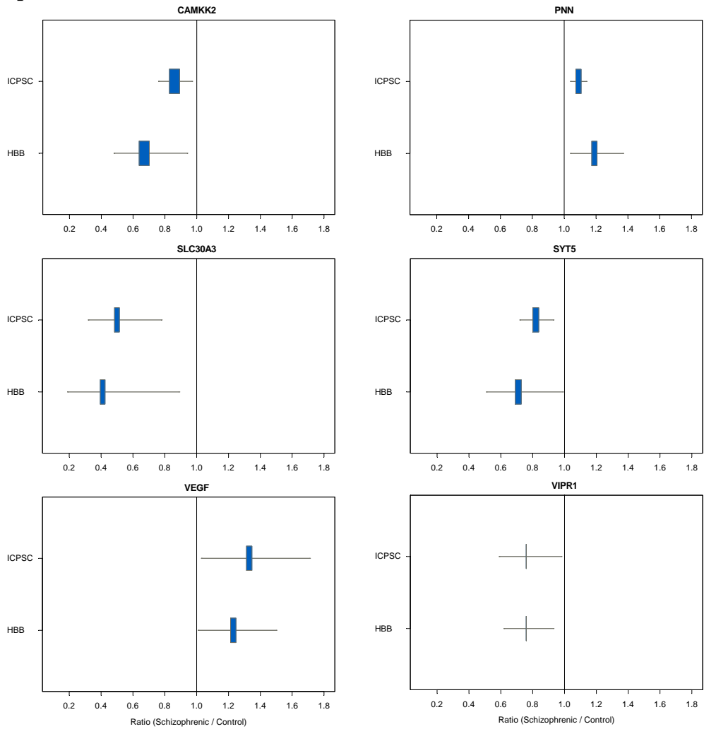
Figure 1: Confidence interval Comparisons
