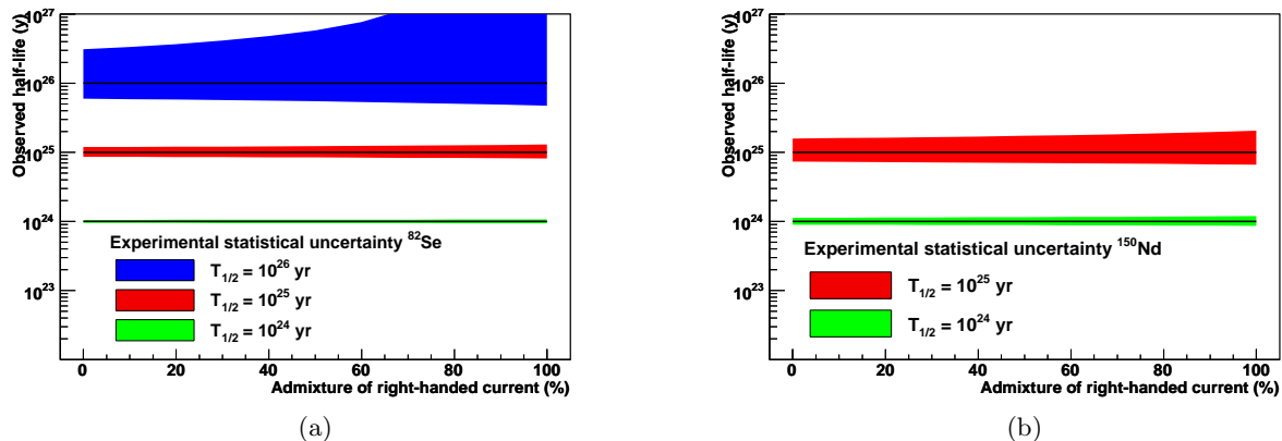
Fig. 8: One standard deviation statistical uncertainties in the measurement of double \beta decay half-lives at SuperNEMO as a function of admixture of the RHC _{\lambda} mechanism represented as band thickness for (a) ^{82}\text{Se} and (b) ^{150}\text{Nd} .
