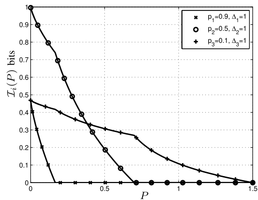
Fig. 5. Individual privacy achieved by three users \mathcal{I}_{X_i}(P) , i = \{1, 2, 3\} , all with the same input load alphabet \delta_i = 1 i = \{1, 2, 3\} , but with different input load distributions as a function of the average AES power P .
