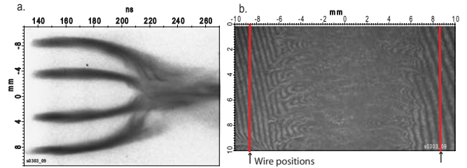
FIG. 4: (a) Radial optical streak photograph showing implosion of a 17 mm diameter, 8 \times 10 \mu\text{m} Al load array. (b) Interferogram of a load array taken 76 ns after current switch showing no trailing mass between the original wire positions (red lines) and the imploding plasma.
