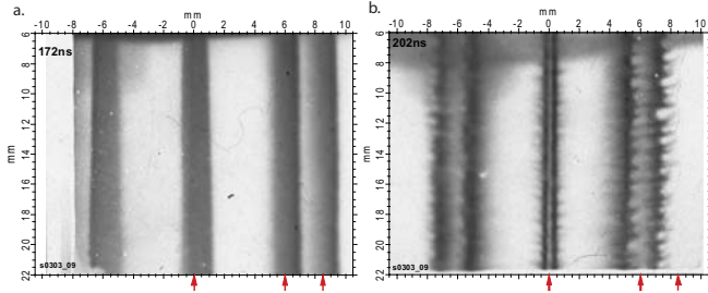
FIG. 5: (a), (b) XUV images showing development of MRT instability during implosion of the load array. Arrows show initial positions of the wires.
