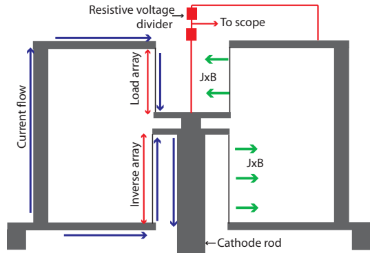
FIG. 1: Diagram of the array configuration with the resistive voltage divider applied.
