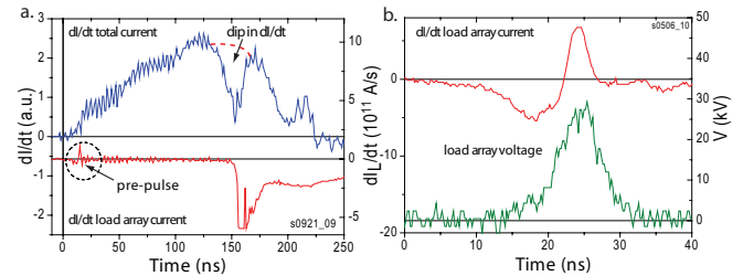
FIG. 2: Plots of (a) the dI/dt of the total current and the current in just the load array and (b) the dI/dt and the resistive voltage across a 17 mm diameter, 8 \times 15 \mu\text{m} Al load array during the pre-pulse.
