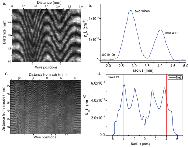
FIG. 3: (a) Interferogram of a load array taken 2 ns before current switch with the measured Al line density ( n_g L ) shown in (b). (c) Interferogram of a load array obtained t \sim 40 ns after current switch with (d) the measured electron line density profile. Red lines indicate initial positions of the wires.
