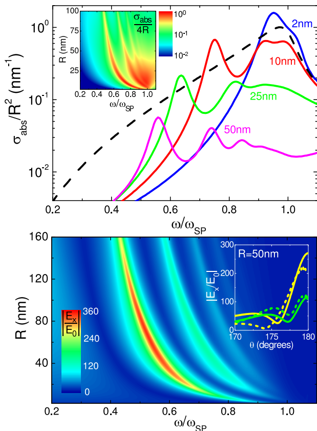
FIG. 4: Upper panel: Absorption cross section normalized to the structure area for Ag ( \beta = 3.6 \times 10^{-3}c ) nanowires of different radius. Color solid lines plot \sigma_{\text{abs}}/R^2 evaluated from Eq. (5) and dashed black line renders the electrostatic local result for all R . The inset shows the absorption efficiency versus the incident frequency and nanowires radius. Lower panel: Absolute value of the field enhancement at the touching point as a function of \omega/\omega_{\text{SP}} and R . Solid (dashed) lines in the inset render theoretical (numerical) |E_x/E_0| at the two lowest enhancement maxima for R = 50 nm: 0.55\omega_{\text{SP}} (yellow), 0.72\omega_{\text{SP}} (green).
