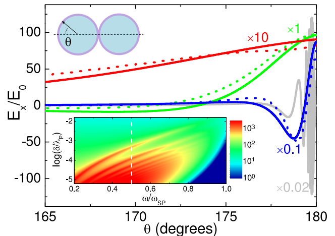
FIG. 2: Field enhancement in the vicinity of the touching point of two 10 nm radii Ag nanowires at \omega = 0.5\omega_{SP} and different degrees of non-locality, \delta/\lambda_P : 10^{-4} (blue), 10^{-3} (green) - this is a realistic value for Ag - and 10^{-2} (red). Solid (dotted) lines show transformation optics (numerical) results. Grey line plots E_x/E_0 under the local description. The inset displays |E_x/E_0| at \theta = 180^\circ as a function of the incident frequency, \omega/\omega_{SP} and \delta/\lambda_P . The white dashed line indicates the operating frequency in the main panel.
