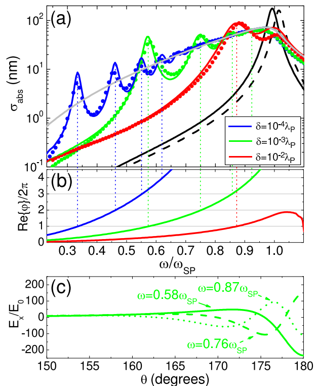
FIG. 3: Panel (a): Theoretical (solid lines) and numerical (dots) absorption spectra for 10 nm radii non-local nanowires, together with the cross section obtained within the local approximation (grey dashed line). \sigma_{\text{abs}} for a local (non-local, \delta = 10^{-2}\lambda_{\text{P}} ) single nanowire is also plotted in solid (dashed) black line. Panel (b): Real part of the phase accumulated by the circulating surface plasmon modes in one loop around the nanowires. (c) Field enhancement close to the touching point at the three lowest non-local resonances for \delta = 10^{-3}\lambda_{\text{P}} (value appropriate for silver).
