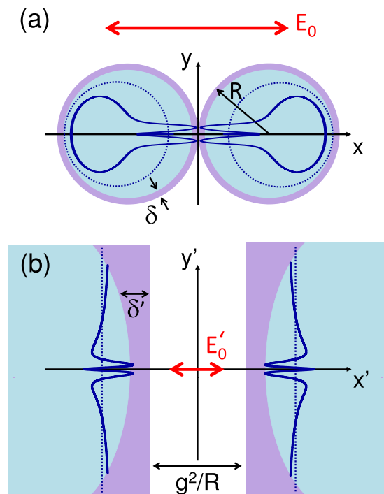
FIG. 1: Panel (a) shows the problem under study: the non-local description of the interaction of light with a dimer of touching metal nanowires. Panel (b) depicts the geometry resulting from the inversion of the original structure. The shaded areas in both panels represent the decay length of the longitudinal plasmons excited in the system. Blue solid lines show artistic plots of the electrostatic potential describing propagating SPPs in both frames.
