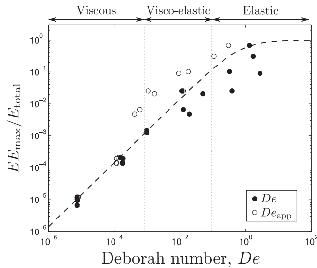
Figure 9. Maximum elastic energy, EE_{max} , scaled to the total strain energy, E_{total} , in the system as a function of the Deborah number, De , for all viscoelastoplastic simulations. Filled circles are measured De , while open circles display the apparent Deborah numbers estimated from the geometric scaling law that we derived for our viscoelastic models (equation (15)). The dashed black line is the energy scaling law previously derived for viscoelastic simulations (see Figure 7). Both De estimates converge for low De where the slabs are too weak to yield, but the apparent Deborah number underestimates the actual De and hence the importance of elasticity if plastic yielding occurs in the slab.
