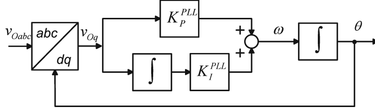
Figure 2: Model for the PLL
