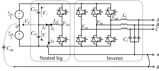
Fig.2: Actively-balanced split-link inverter.
