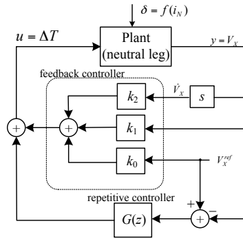
Fig.5. The control system. A deadbeat feedback controller and a repetitive controller are connected in parallel.
