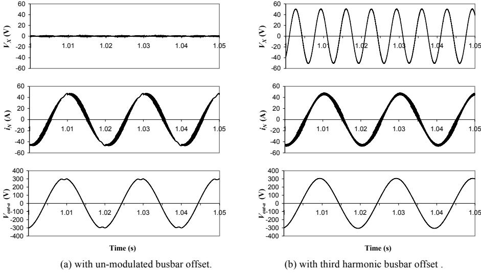
Fig.6: Simulation results. From top to bottom: busbar offset voltage, V_X ; neutral current, i_N ; and phase- a output voltage after the LC filter, V_{Aa} .
