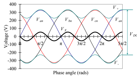
Fig.4 Illustration of reduced V_{DC} when V_X is third harmonic.
