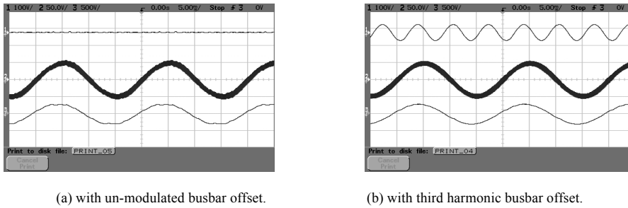
Fig.7: Experimental results. From top to bottom: busbar offset voltage, V_X , 100V/div (measured with potential divider of two 47 k \Omega resistors between V_+ and V_- busbars); neutral current, i_N , 50A/div and phase- a output voltage after the LC filter, V_{Aa} , 500V/div. Time axis is 5 ms/div
