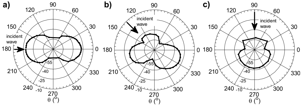
Figure 2.4: The amplitude of 950 kHz-mm S0 scatter from 15 mm long, 2 mm wide through thickness notches oriented along 90^{\circ} - 270^{\circ} on a 3.18 mm thick aluminum plate which result with the interaction of waves that propagate 500 mm in the directions indicated by the arrows to the notch and 500 mm onwards to monitoring points. Results are adapted from [47], and are shown as dB values normalized by the amplitude of the input being at incident angles of (a) 0^{\circ} , (b) -45^{\circ} , and (b) -90^{\circ} .
