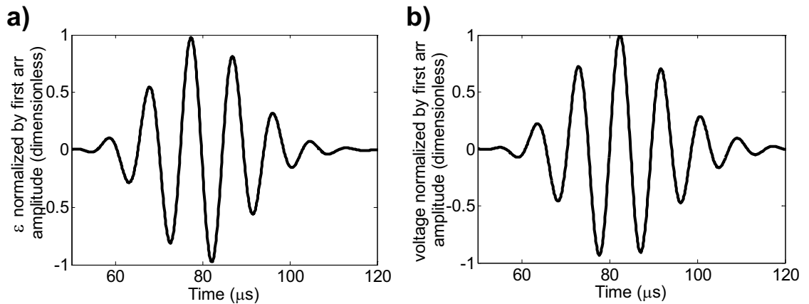
Figure D.2: (a) Strain signal \epsilon(t) of the S0 arrival at p = 0.42 m which was estimated using outputs from simulations with the model of Figure D.1(a) and (b) the wavepacket at the S0 arrival in the received signal computed using monitored voltage responses from simulations with the model of Figure D.1(b); results are normalized to have unity amplitude.
