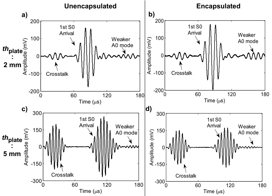
Figure 3.12: Pitch catch data obtained using (a) unencapsulated and (b) encapsulated 20 mm diameter, 0.5 mm thick PZTs bonded on a 2 mm thick, 1.25 m square aluminum plate with separations of 300 mm in the configuration of Figure 3.11(a) and (c)-(d) the data obtained using the 1 mm thick PZTs bonded with separations of 420 mm in the configuration of Figure 3.11(a) on the 5 mm thick plate; the tonebursts used in Figure 3.9 were applied to the transmitting PZTs.
