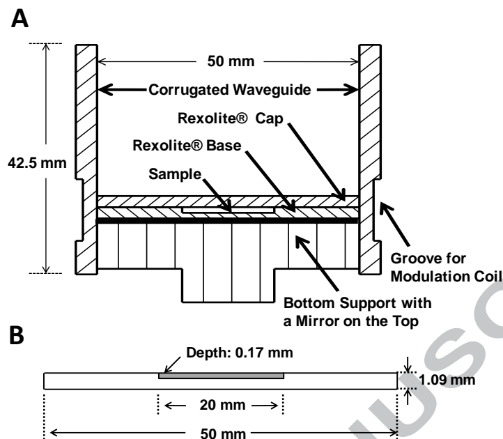
Figure 1. (A) Schematic diagram of the HiPER thin-layer sample holder (See details in section 2.6.). (B) Closer view of the thin-layer recessed sample space of the holder H2.
