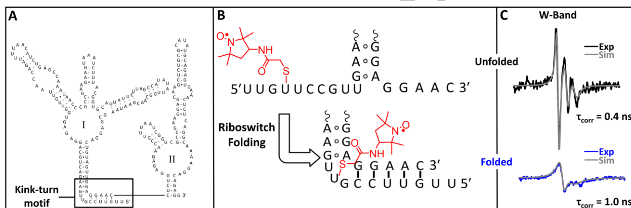
Figure 4. (A) Secondary structure of the 232 nt VC glycine riboswitch with the kink-turn motif boxed in black. (B) Enlarged kink-turn motif structure depicted in the unfolded (top) and folded (bottom) states showing IAP on the chosen modified thiouridyl base. (C) Experimental and simulated (grey) W-Band spectra for the unfolded (top, black) and folded (bottom, blue) riboswitch states with signal to noise ratios for each shown. The arrow indicates features in the folded state spectrum that may arise from a small fraction of unfolded RNA (< 1%) Spectra were collected using 200 G sweep width, 1 second time constant, 4 G modulation amplitude, and 5 (unfolded) and 6 (folded) averages.
