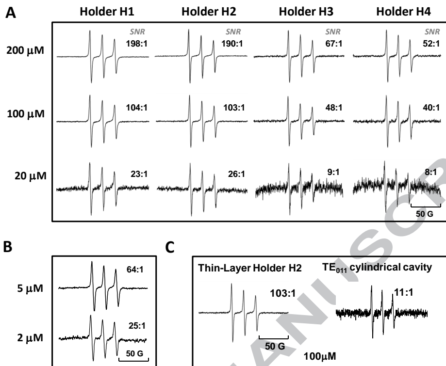
Figure 2. (A) Absorption area normalized EPR spectra of TEMPO solutions using different thin-layer sample holders. Spectra are vertically offset for clarity. Spectra were collected using 150 Gauss sweep width, 1 Gauss modulation-amplitude, 100 millisecond time constant, and 1 average at room temperature (75 second scans). SNRs are marked in the upper-right corners of the spectra. (B) Spectra of 2 \mu\text{M} and 5 \mu\text{M} TEMPO using sample holder H2. Both spectra were collected using 150 Gauss sweep width, 2 Gauss modulation-amplitude, 1 second time constant, and 6 averages (13 minute scans) at room temperature. (C) Spectra of 100 \mu\text{M} TEMPO using holder H2 on HiPER and a \text{TE}_{011} cylindrical cavity on a Bruker E680 spectrometer. Comparable parameters were chosen as follows: (i) HiPER holder H2: 1 Gauss modulation amplitude, 100 millisecond time constant, 100 millisecond conversion time, 150 Gauss sweep width, and one scan (75 seconds); (ii) \text{TE}_{011} cylindrical cavity: 1 Gauss modulation amplitude, 80 millisecond time constant, 80 millisecond conversion time, 150 Gauss sweep width, and one scan (82 seconds). Note: slightly different time constants were used for the two spectrometers because of the different setups of their lock-in amplifiers.
