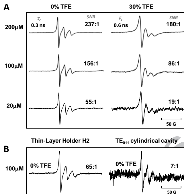
Figure 3. Intensity normalized W-band spectra of SL-IA 3 at site E10P1. (A) Spectra are vertically offset showing how values of the SNR change as a function of concentration with 0% and 30% TFE at 300 K. Spectra were collected using sample holder H2 with 200 G sweep width, 2 G modulation-amplitude, 1 second time constant and 6 averages (13 minute scans). The spectral line shape and rotational correlation time changes for the 0% and 30% TFE states are consistent with an unstructured to helical transition (simulated spectra are given in Supporting Information). (B) Comparison of concentration sensitivity of the H2 holder on HiPER and a TE 011 cylindrical cavity on a Bruker E680 spectrometer. Spectra are acquired for a 100 μM sample. Comparable spectral parameters were utilized as follows: (1) HiPER holder H2: 2 G modulation amplitude, 1 second time constant, 1 second conversion time, 200 G sweep width, and one scan (17 minutes). TE 011 cylindrical cavity: 2 G modulation amplitude, 1.3 second time constant, 1.3 second conversion time, 200 G sweep width, and one scan (22 minutes). Note: slightly different time constants were used for the two spectrometers because of the different setups of their lock-in amplifiers.
