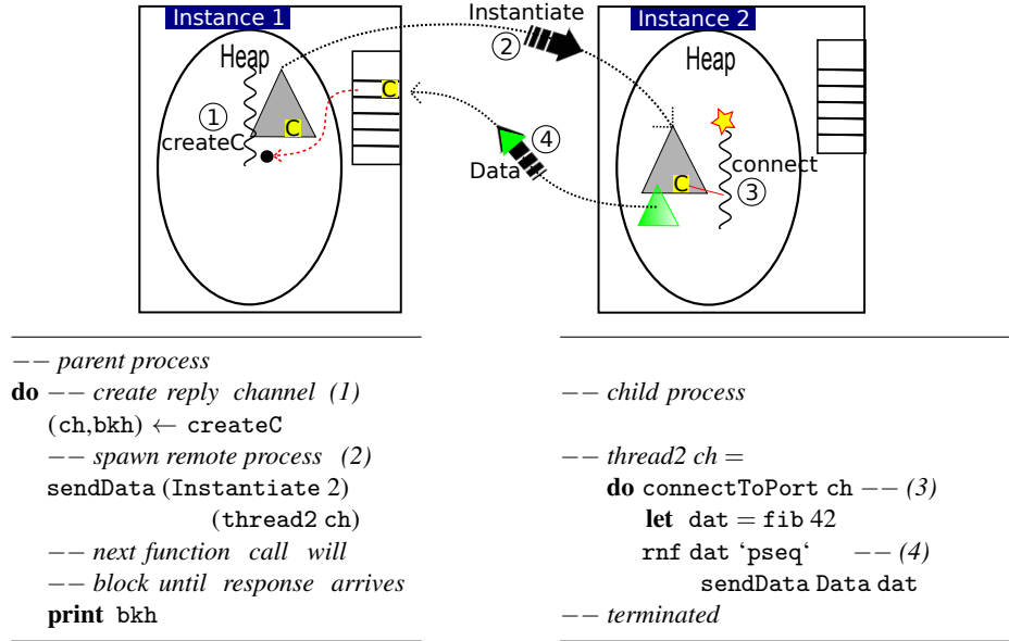
Fig. 13. Communicating computations and values explicitly. A thread on Instance 1 creates a channel (1) and passes the created ChanName to a new process on Instance 2 (2). A newly created thread connects to the channel (3) and sends evaluated Data (4).
