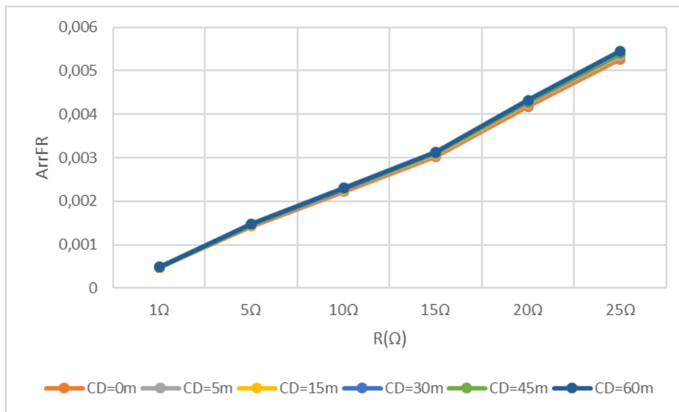
Figure 6.32: Failure Rate of the arrester installed at position D_{in} in function with the Grounding Resistance and the distance between the arrester and the transformer (CD) considering BD=300m (case b)
