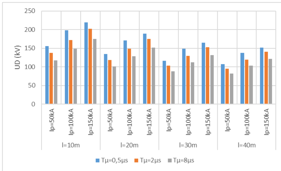
Figure 7.8 Induced Overvoltages at the position D for lightning bit on position K for various current waveforms (case a)
