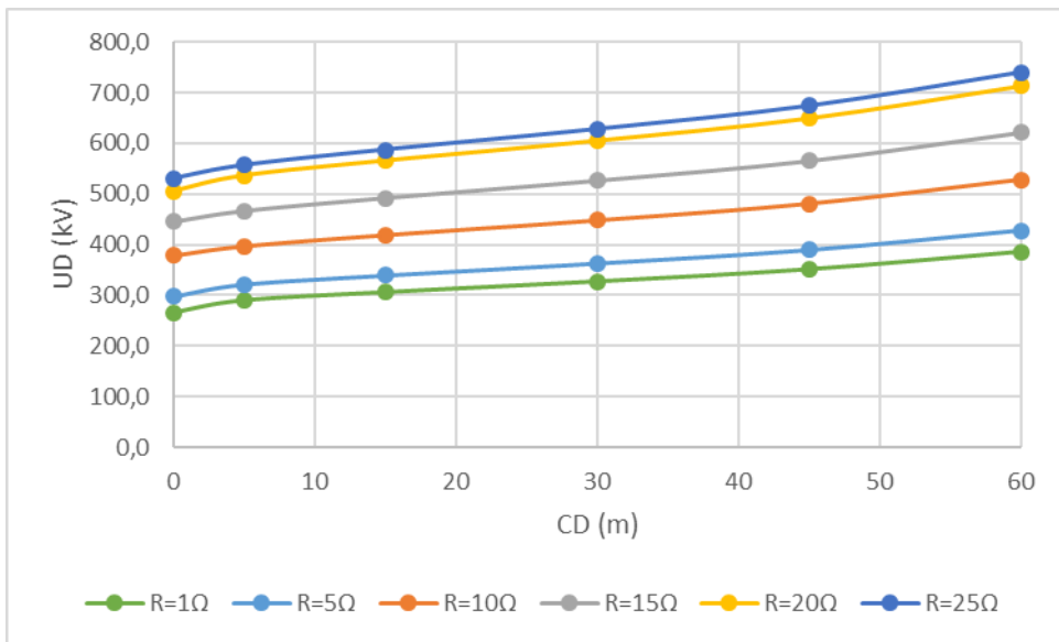
Figure 5.14: The Developed Overvoltage at Position D (UD) in function with the Distance CD and the Tower Footing Resistance (Lightning hit on the Ground Wire of the Connected Transmission Line, BD=600m , case a)
