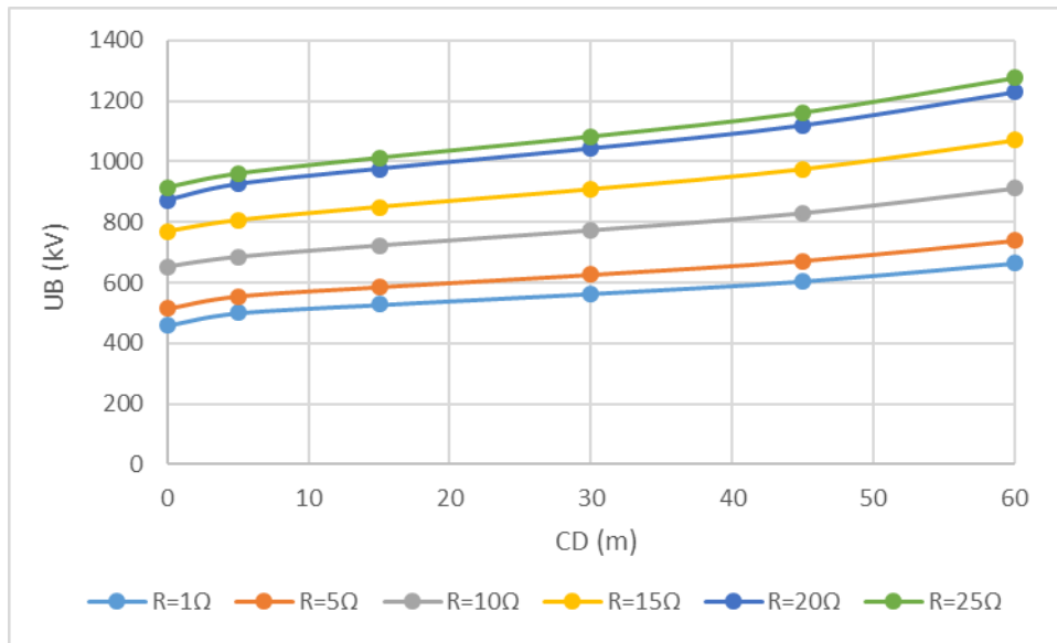
Figure 5.29: The Developed Overvoltage at Position B ( U_B ) in function with the Distance CD and the Tower Footing Resistance (Lightning bit on the Ground Wire of the Connected Transmission Line, BD=1000m , case b)
