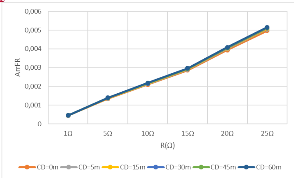
Figure 6.35: Failure Rate of the arrester installed at position D_{in} in function with the Grounding Resistance and the distance between the arrester and the transformer (CD) considering BD=2000m (case b)
