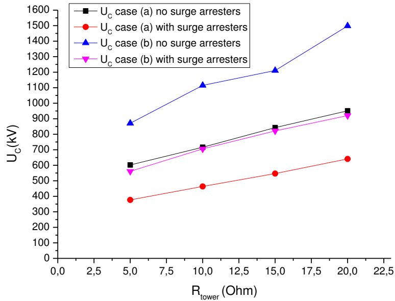
Figure 5.52: Overvoltage at Position C ( U_c ) in function with Grounding Resistance for Direct (case (I)) or Indirect (case (II)) Lightning hit for the Topology of Figure 4.2, Protected or Not by Surge Arresters
