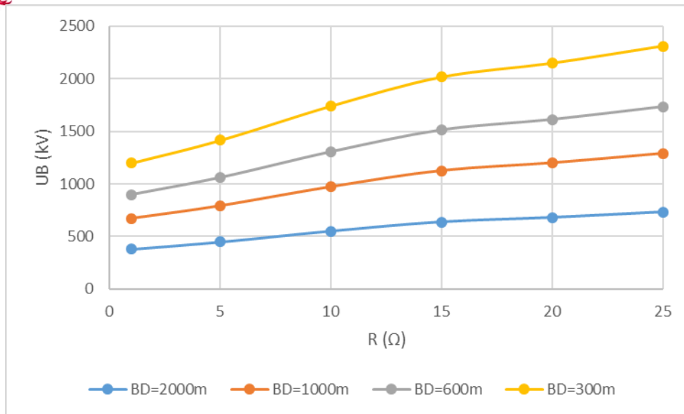
Figure 5.12: The Developed Overtoltage at Position B ( U_B ) in function with the Tower Footing Resistance (Lightning hit on the Ground Wire of the Connected Transmission Line, No Arresters Installed)
