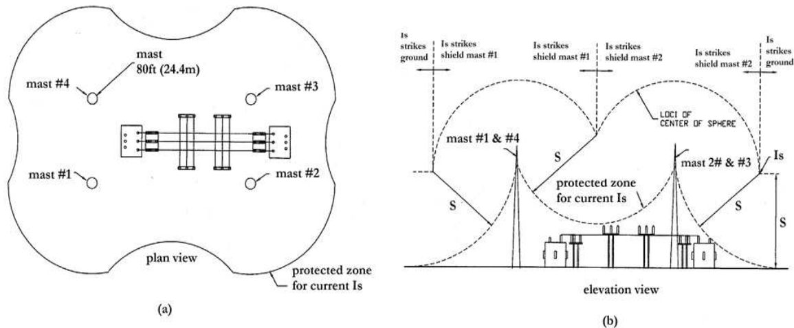
Figure 3.24: Multiple Shield Mast Protection for Stroke Current I_s (McDonald et al. 2000, IEEE Std 998-1996)
