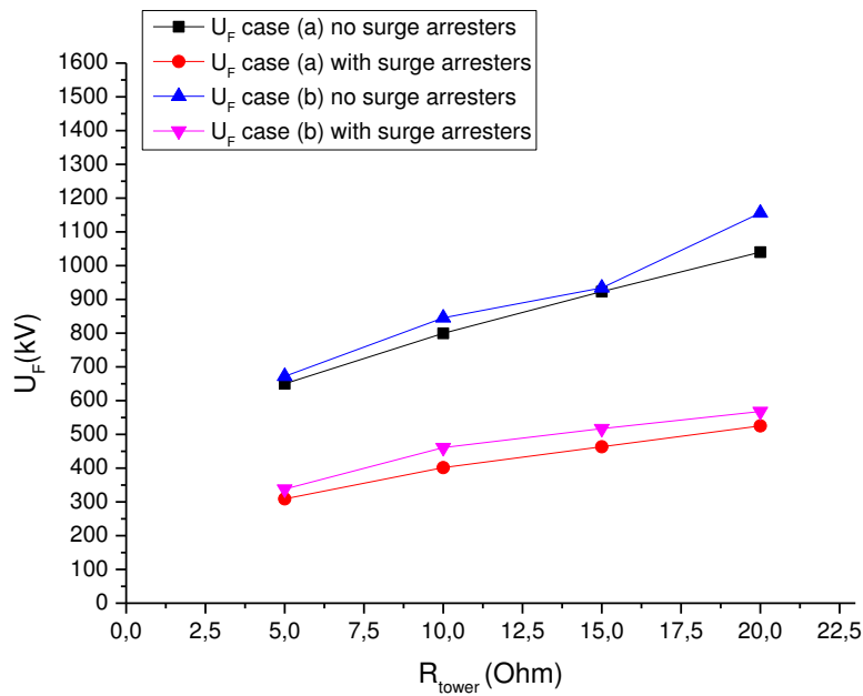
Figure 5.55: Overvoltage at Position F ( U_F ) in function with Grounding Resistance for Direct (case (I)) or Indirect (case (II)) Lightning hit for the Topology of Figure 4.2, Protected or Not by Surge Arresters
