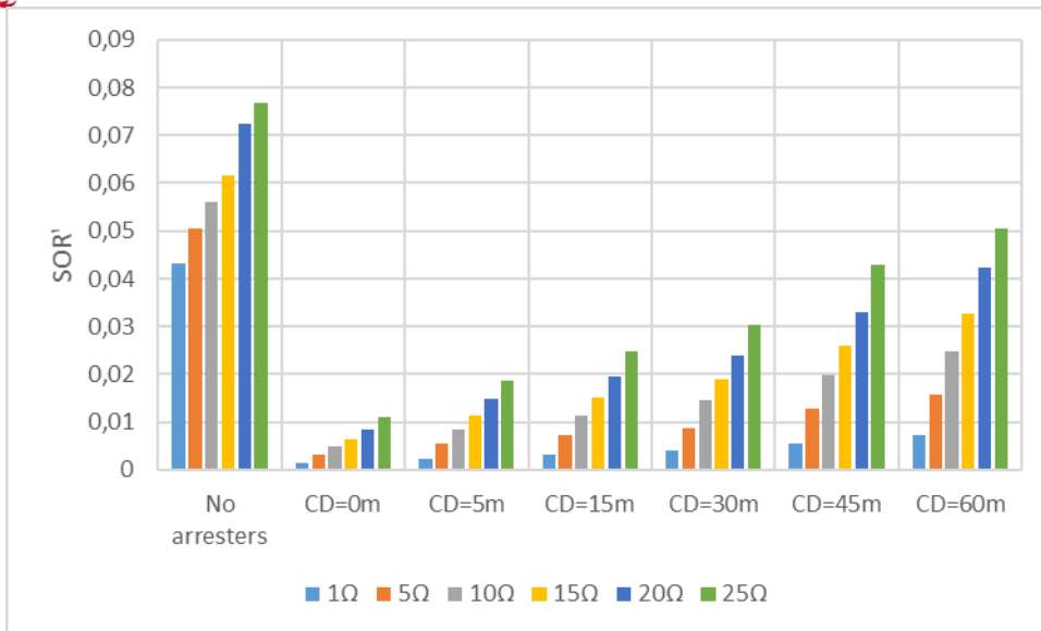
Figure6.39: Substation Outage Rate including Arresters Faults in function with the Grounding Resistance and the distance between the arresster and the transformer (CD) considering BD=2000m (case b)
