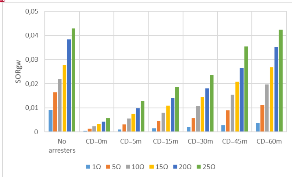
Figure 6.27: Substation Outage Rate in case of lightning bit on ground wire of the connected line in function with the grounding resistance (R) and the distance between the arrester and the transformer (CD) considering BD=2000m (case b)
