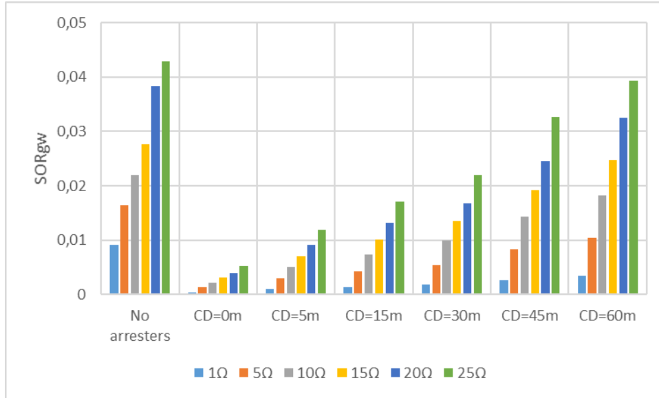
Figure 6.5: Substation Outage Rate in case of lightning hit on ground wire of the connected line in function with the grounding resistance (R) and the distance between the arrester and the transformer (CD) considering BD=2000m (Case a)
