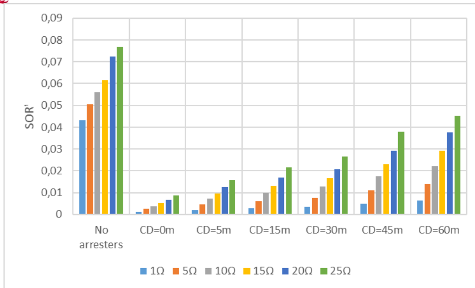
Figure6.21: Substation Outage Rate including Arresters Faults in function with the Grounding Resistance and the distance between the arrester and the transformer (CD) considering BD=2000m (Case a)
