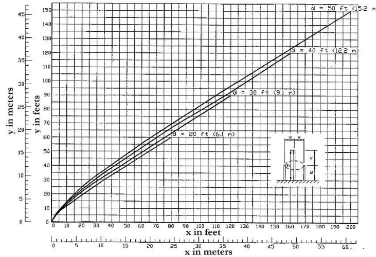
Figure 3.20: Single lightning Mast Protecting Single Ring of Object—0.1% Exposure. (y: Height of Mast above Protected Object, s: Horizontal Separation, d: Height of Protected Object) (McDonald et al. 2000, IEEE Std 998-1996)
