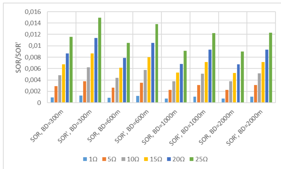
Figure6.22: Comparison Substation Outage Rate including and not including Arresters Faults in function with the Grounding Resistance and the distance and the length of the cable (BD) considering CD=0m (Case a)
