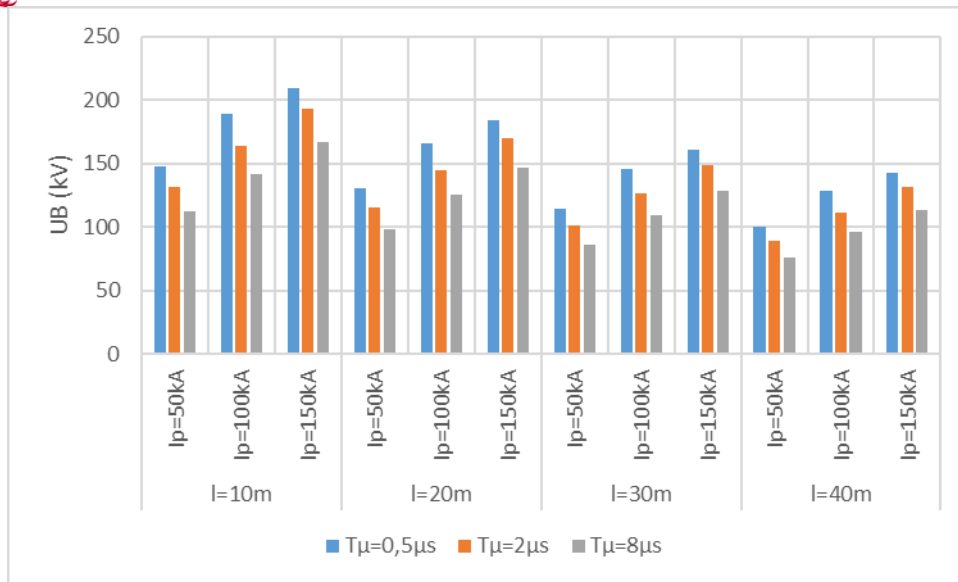
Figure 7.7 Induced Overvoltages at the position B for lightning bit on position K for various current waveforms (case a)
