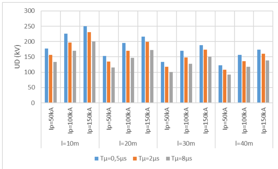
Figure 7.14 Induced Overvoltages at the position D for lightning bit on position K for various current waveforms (case b)
