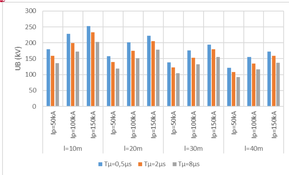
Figure 7.13 Induced Overvoltages at the position B for lightning bit on position K for various current waveforms (case b)
