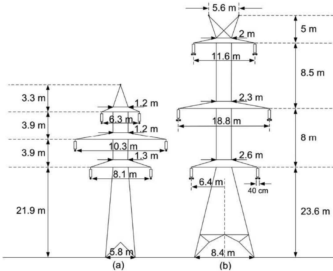
Figure 3.7: Typical Towers of :(a) 150 kV, (b) 400 kV Double-Circuit Lines; the length of insulator strings are 1.86 (m) and 3.62 (m) for the 150 kV and 400 kV line, respectively (Mikropoulos et al. 2010)
