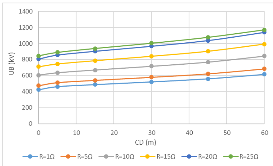
Figure 5.30: The Developed Overvoltage at Position B ( U_B ) in function with the Distance CD and the Tower Footing Resistance (Lightning bit on the Ground Wire of the Connected Transmission Line, BD=2000m , case b)
