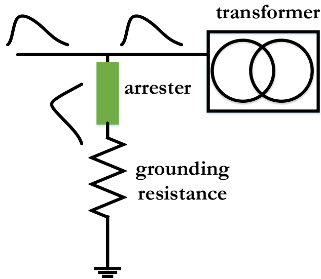
Figure 5.3: Power Transformer protected by Surge Arresters
