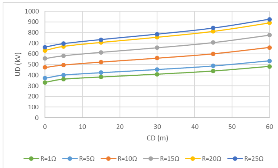
Figure 5.24: The Developed Overvoltage at Position D (UD) in function with the Distance CD and the Tower Footing Resistance (Lightning hit on the Ground Wire of the Connected Transmission Line, BD=600m , case b)
