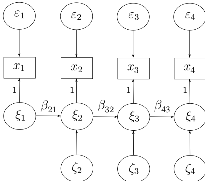
Figure 1: Path diagram of a four-wave quasi-Markov simplex model
