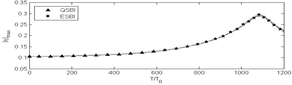
Fig. 10. The exchange between the models (solid line represents the values of |\eta|_{max} )
