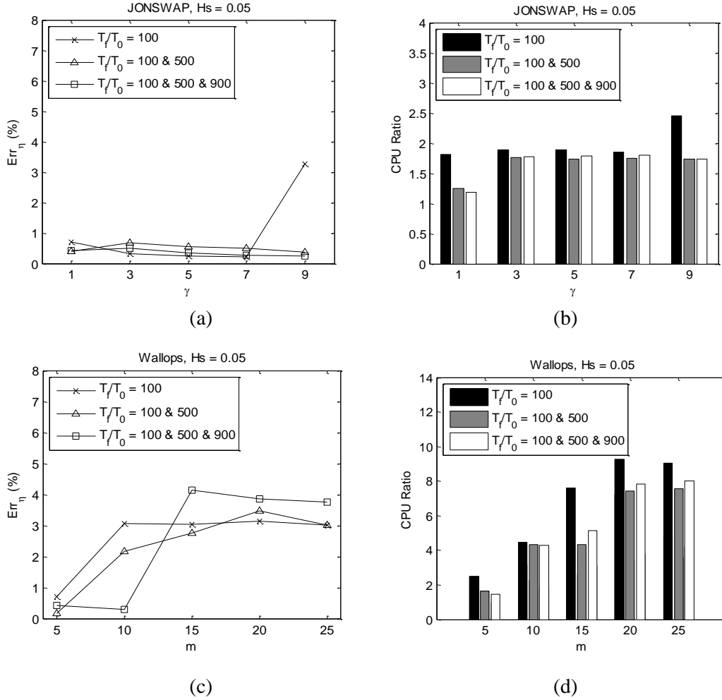
Fig. 14. Err_n and CPU ratio (CPU time of ESBI/CPU time of hybrid model) for the cases of different amount of rogue waves on temporal scale
