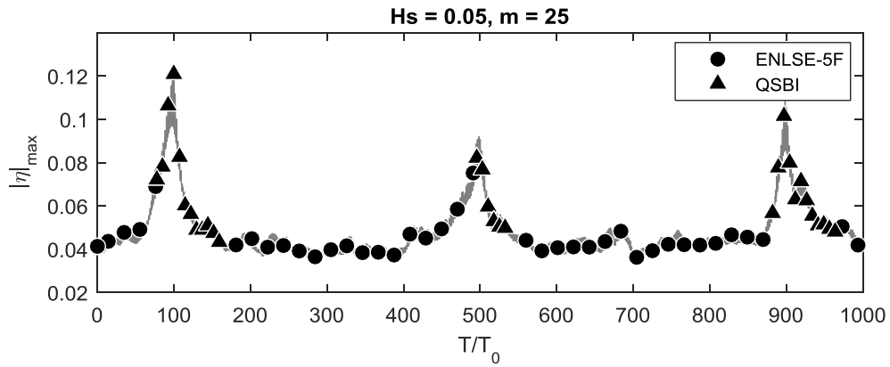
Fig. 15. Maximum wave elevations with indicator which model is used for the cases of different numbers of rogue waves in time domain
