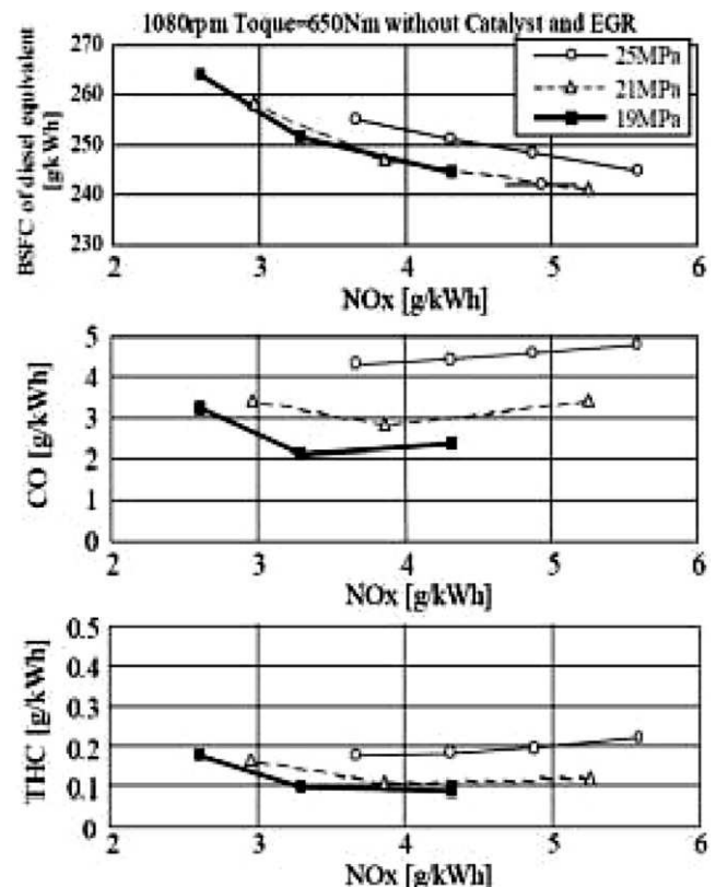
Fig. 5. Effect of fuel-injection pressure in the low speed and high load operating conditions for DME with a single cylinder of 638 ml DI compression-ignition engine [18].
