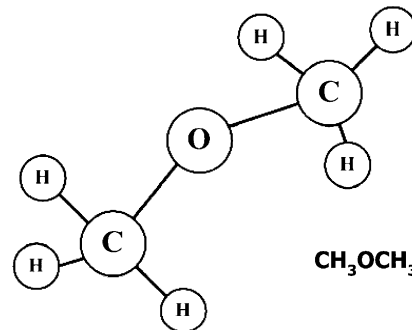
Fig. 1. Structure of di-methyl ether (DME).
