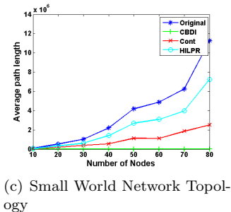
Figure 4: Average Path Length versus the number of nodes and \alpha , for the Original network and when nodes are removed using the CBDI , Cont and HILPR algorithms, in three different network topologies.
