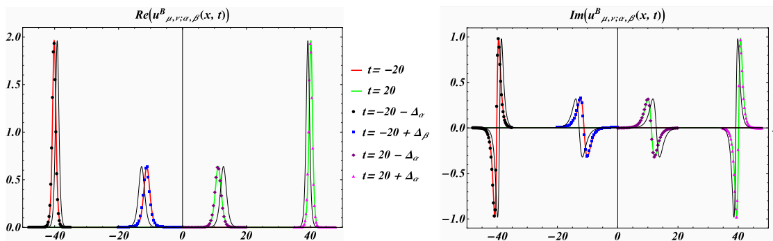
Figure 2: Time delay in the KdV complex two-soliton scattering u_{\mu,\nu;\alpha,\beta}^B for \mu = \nu = i\pi/2 , \alpha = 7/5 and \beta = 4/5 . The scattered solitons are the one-soliton solutions at the shifted times as indicated in the legend and the thin solid black lines are the unshifted one-soliton solutions at time t = -20, -20, 20, 20 from the left to the right.
