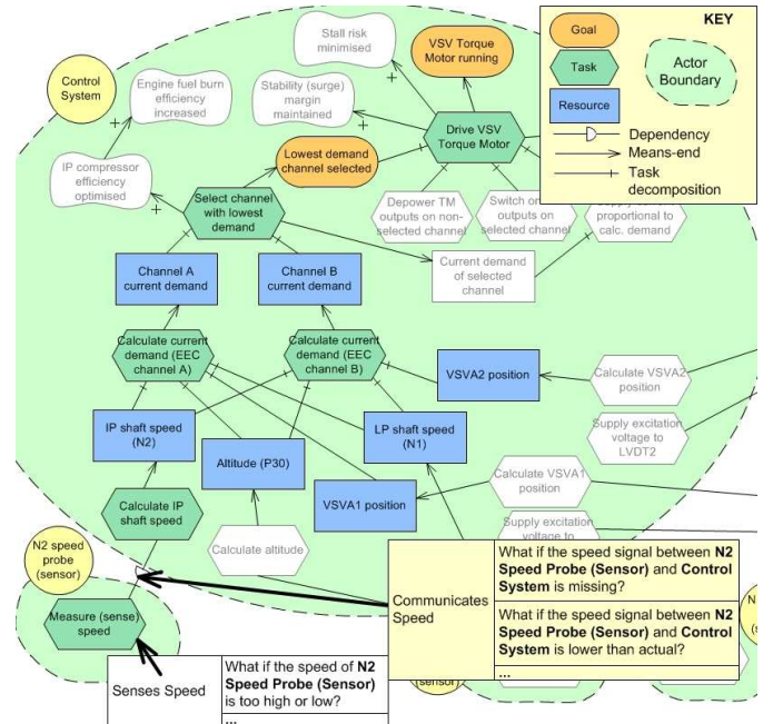
Figure 2: An i^* Strategic Rationale model of the VSV system showing the impact of selected abnormal scenario events on the completion of actor tasks and the validity of actor dependencies
