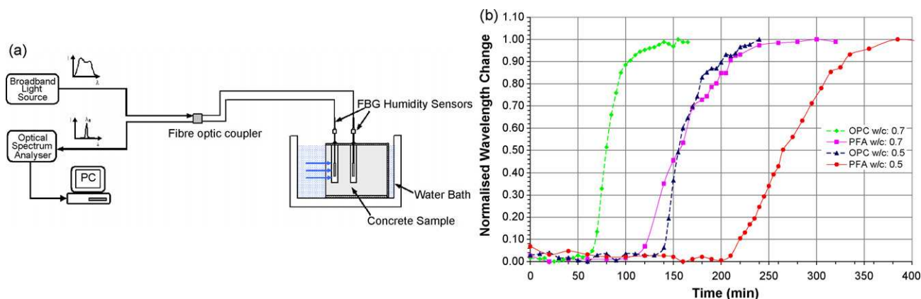
Fig. 12. (a) Experimental set-up used for moisture ingress rate measurement using FBG humidity sensors. (b) Sensor measurements showing moisture ingress characteristics of various concrete specimens using sensor positioned at 25 mm away from cube face [62].
